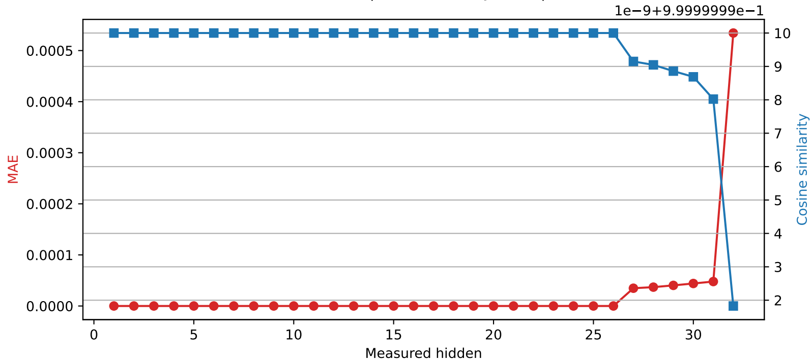
Mistral-7B-Instruct-v0.3 | Quantized layer 26 | float32 → int16
