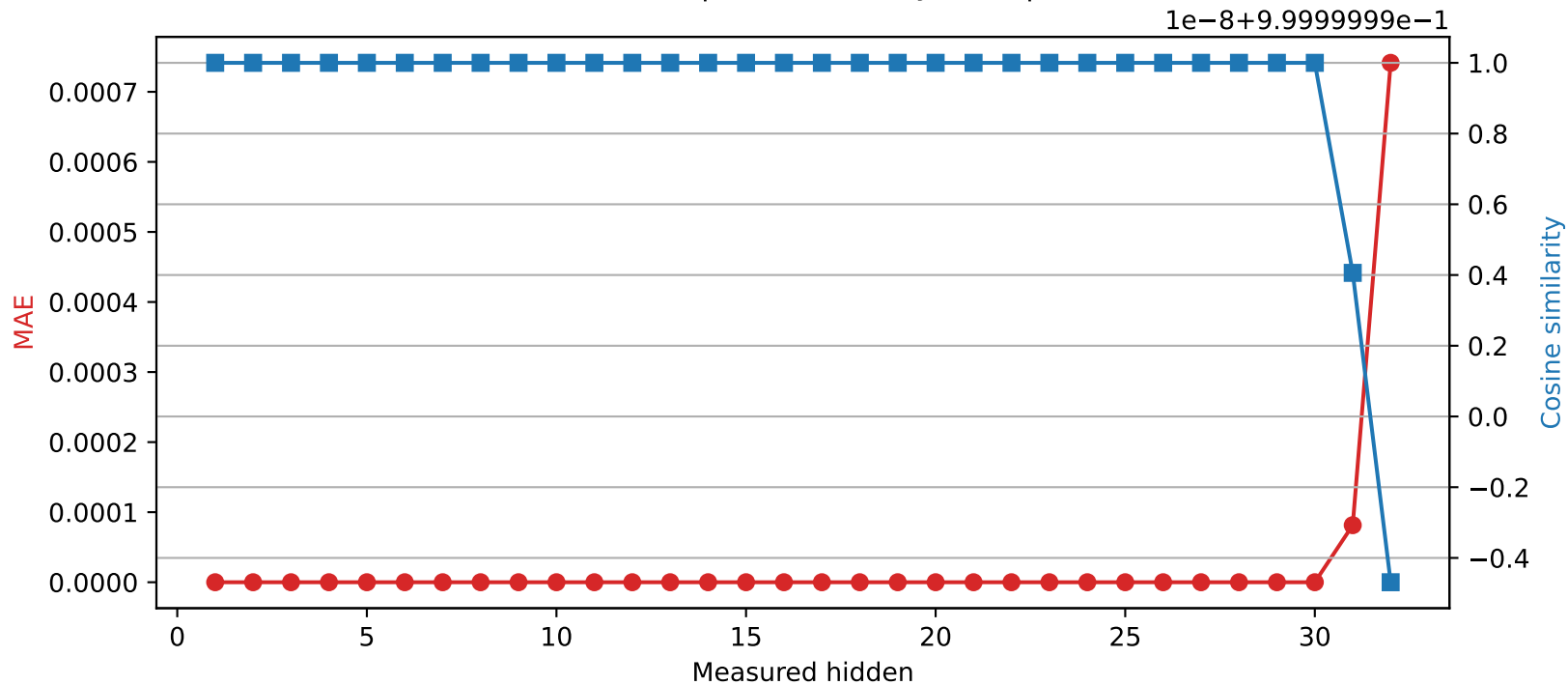
Mistral-7B-Instruct-v0.3 | Quantized layer 30 | float32 \rightarrow int16
