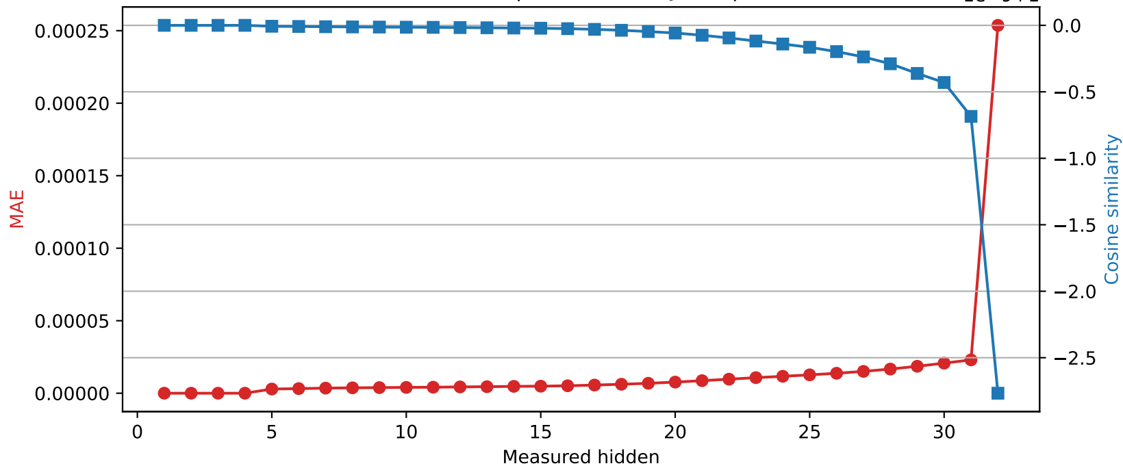
Mistral-7B-Instruct-v0.3 | Quantized layer 4 | float32 → int16
