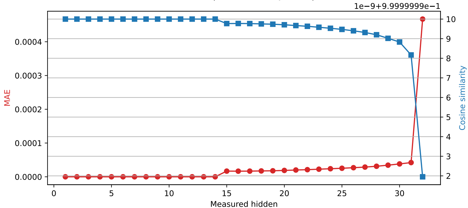
Mistral-7B-Instruct-v0.3 | Quantized layer 14 | float32 → int16
