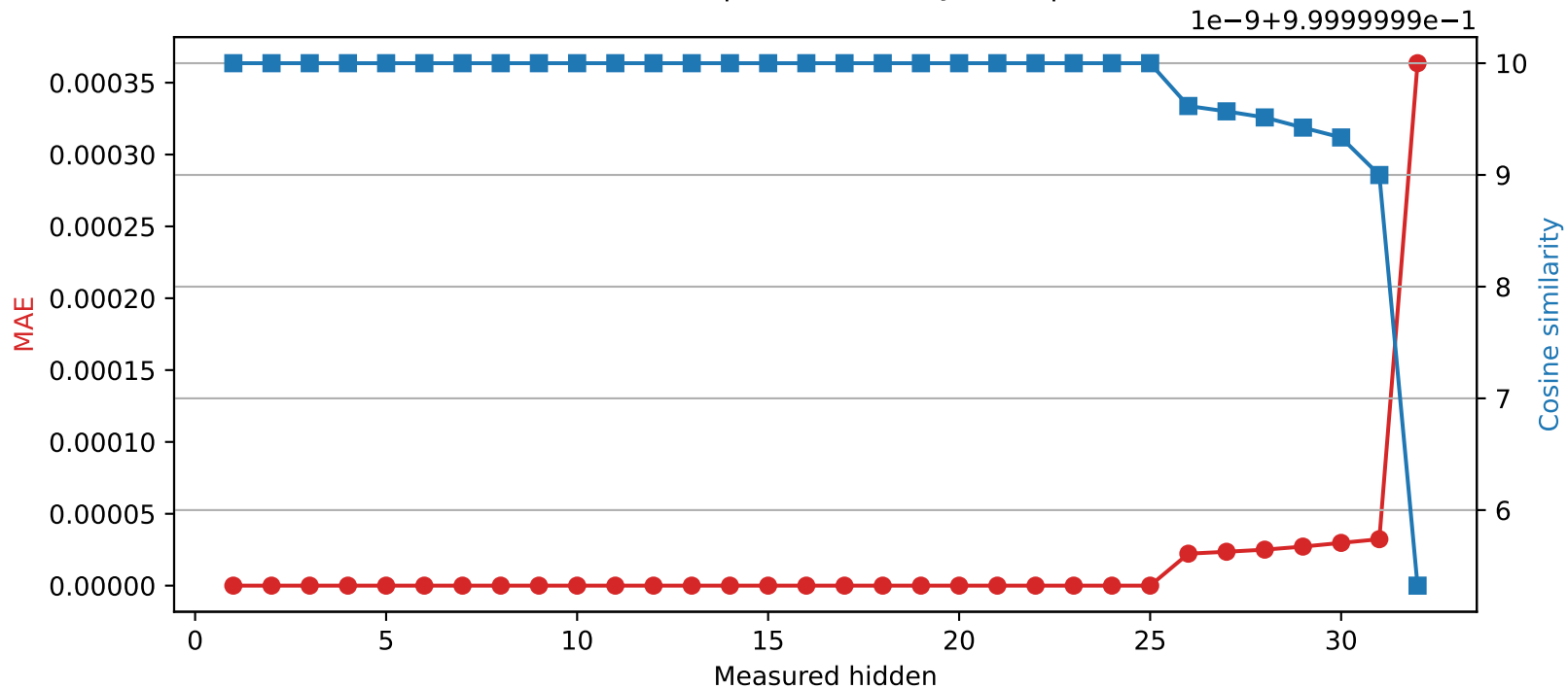
Mistral-7B-Instruct-v0.3 | Quantized layer 25 | float32 → int16
