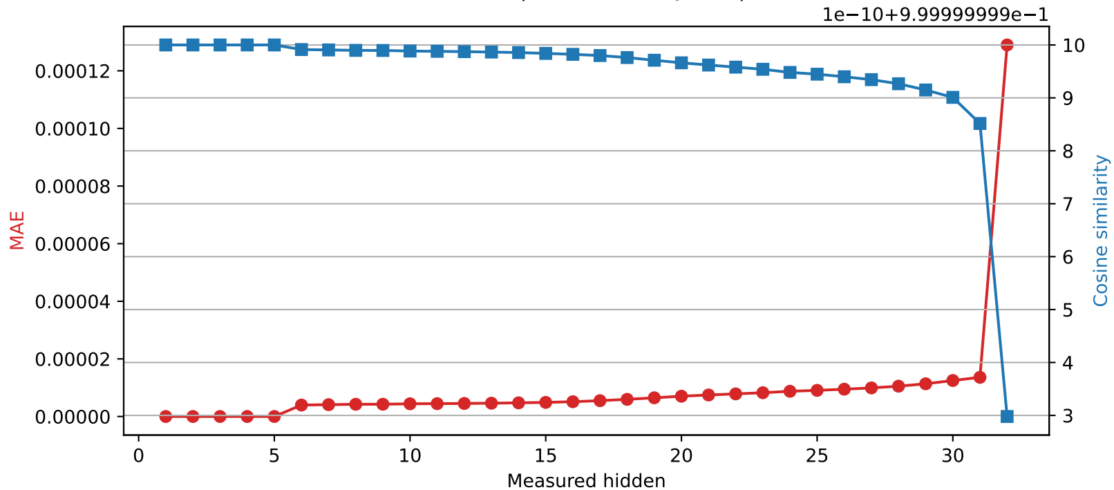
Mistral-7B-Instruct-v0.3 | Quantized layer 5 | float32 \rightarrow int16
