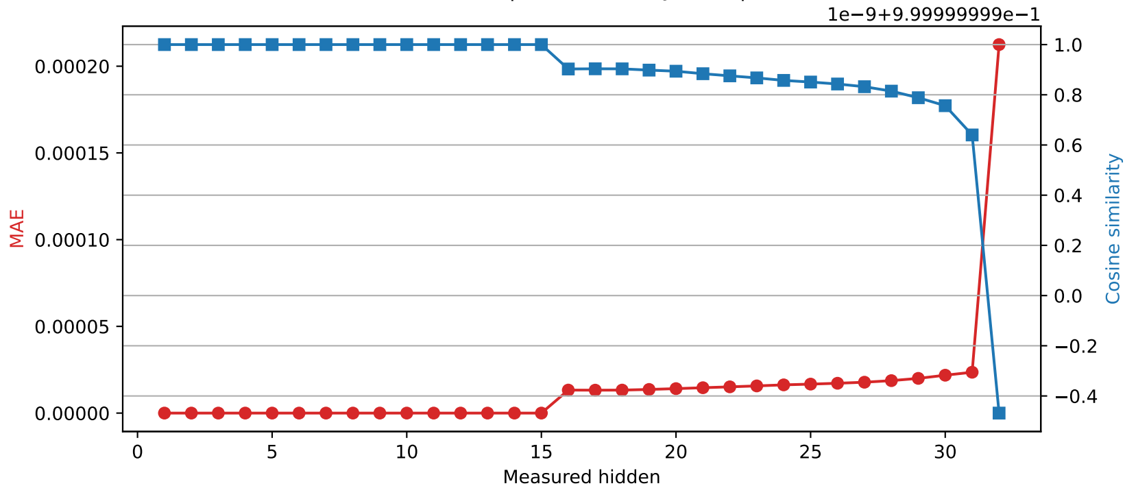
Mistral-7B-Instruct-v0.3 | Quantized layer 15 | float32 → int16
