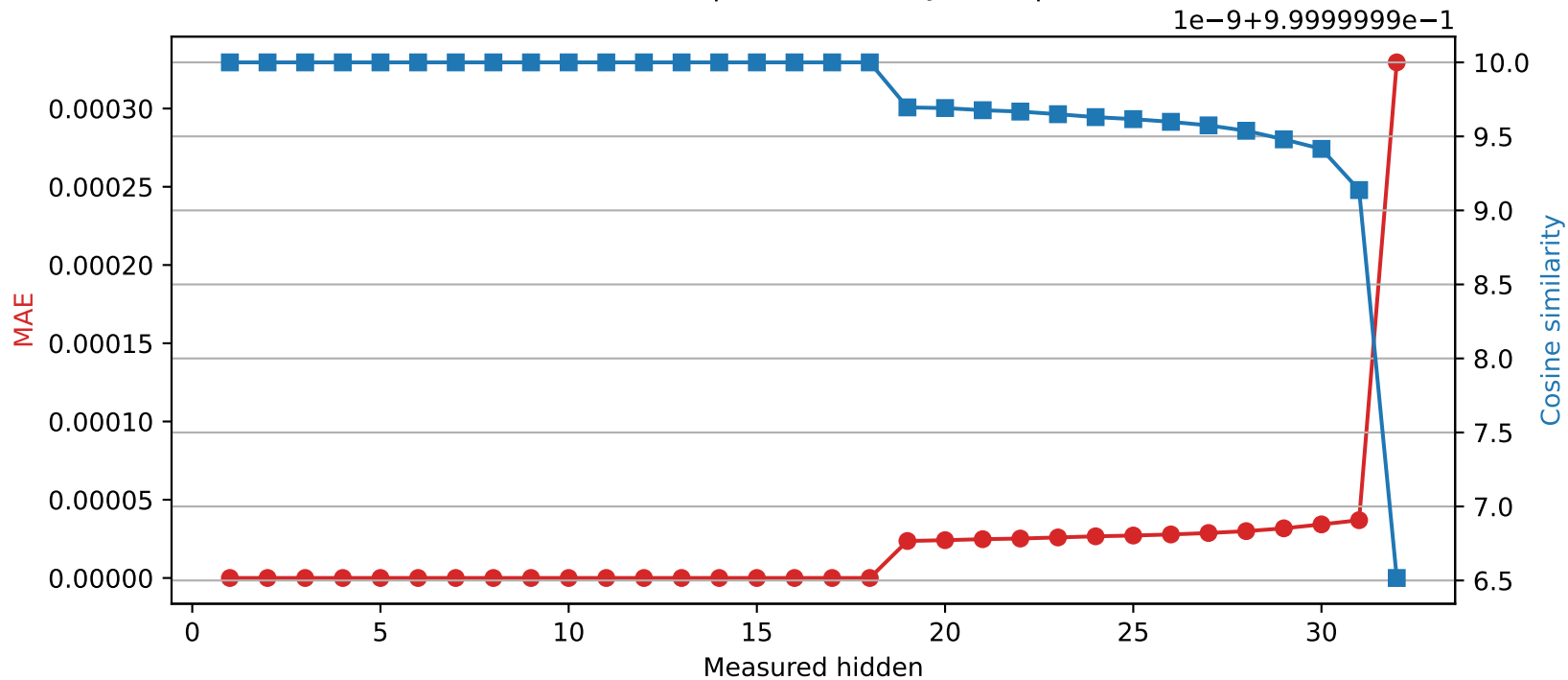
Mistral-7B-Instruct-v0.3 | Quantized layer 18 | float32 \rightarrow int16
