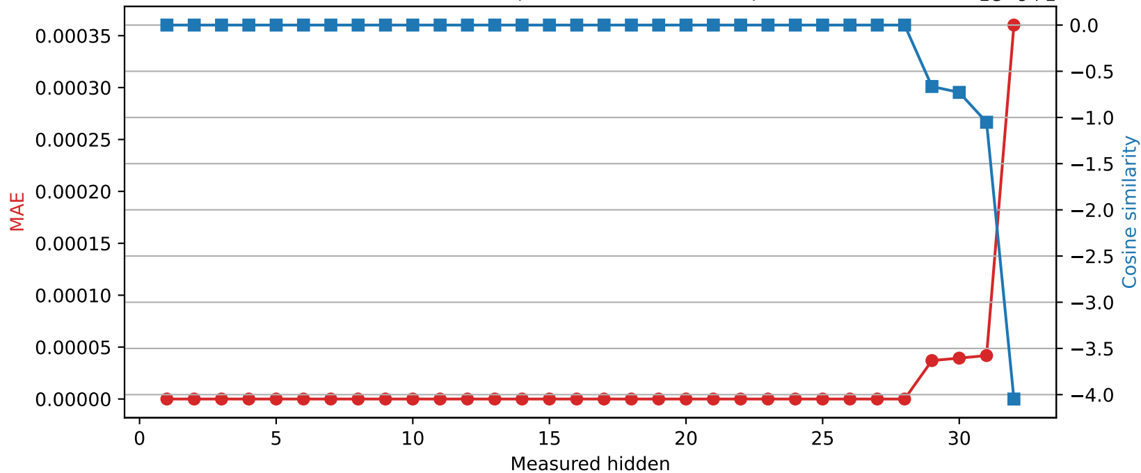
Mistral-7B-Instruct-v0.3 | Quantized layer 28 | float32 → int16
