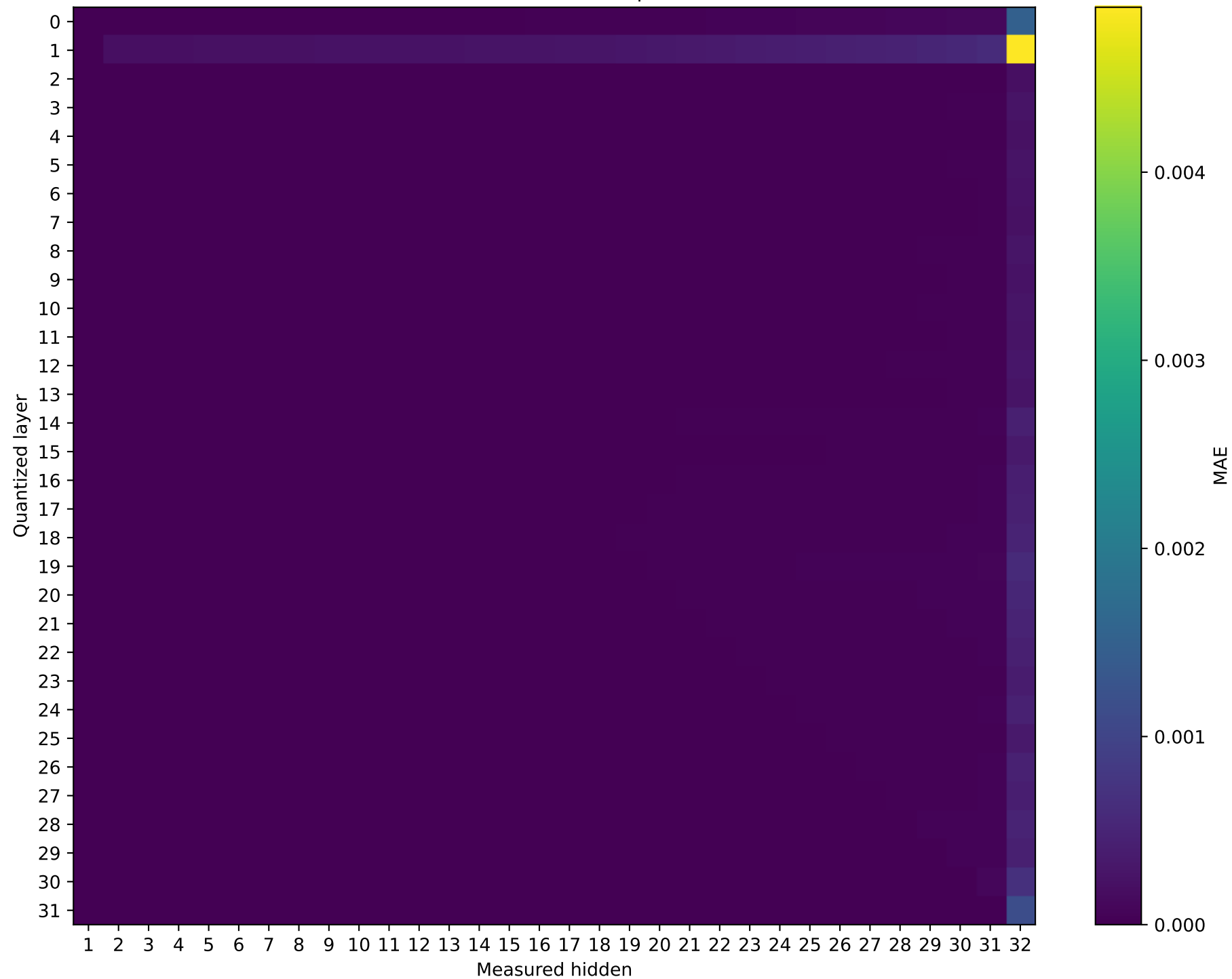
Model: Mistral-7B-Instruct-v0.3 | float64 → int16
