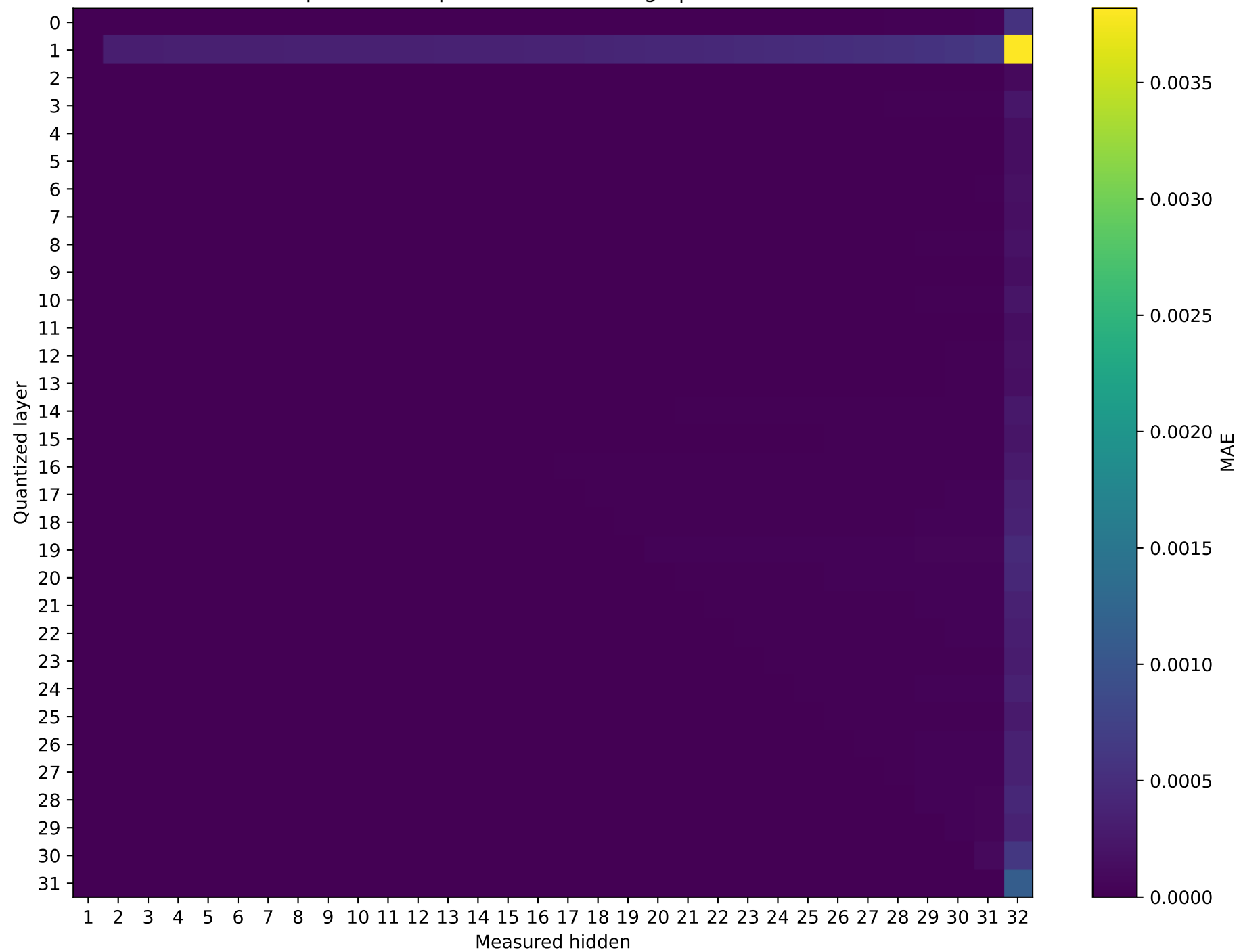
Mistral-7B-Instruct-v0.3 Prompt 0: MAE representation damage | float64 → int16
