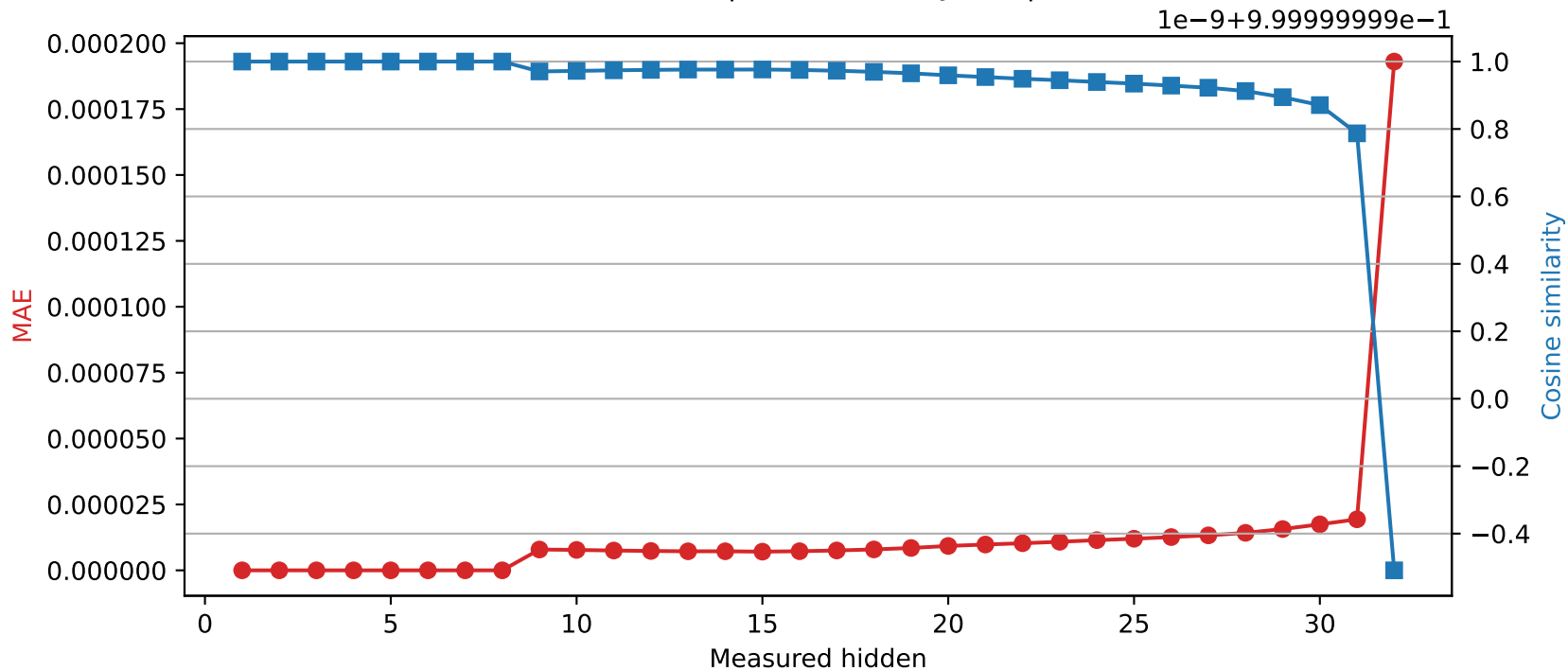
Mistral-7B-Instruct-v0.3 | Quantized layer 8 | float64 → int16
