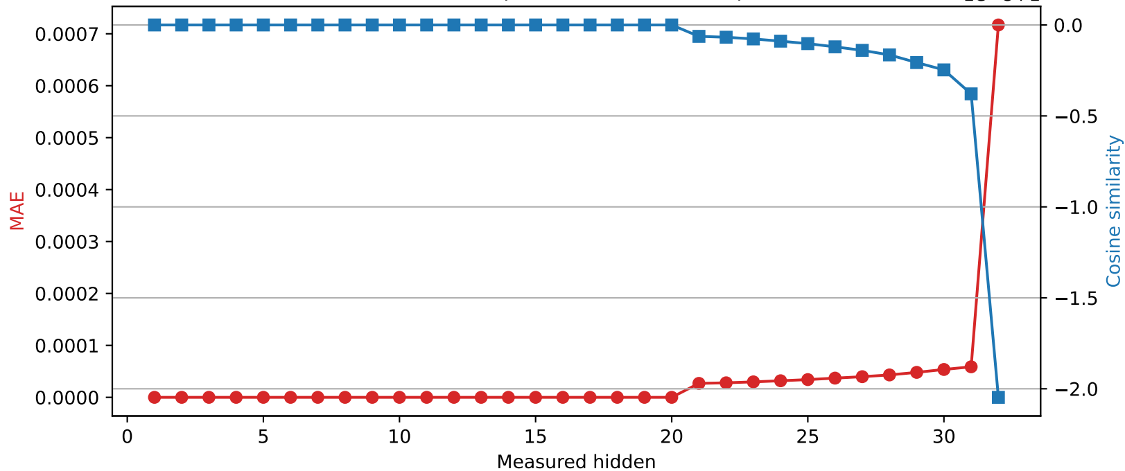
Mistral-7B-Instruct-v0.3 | Quantized layer 20 | float64 → int16
