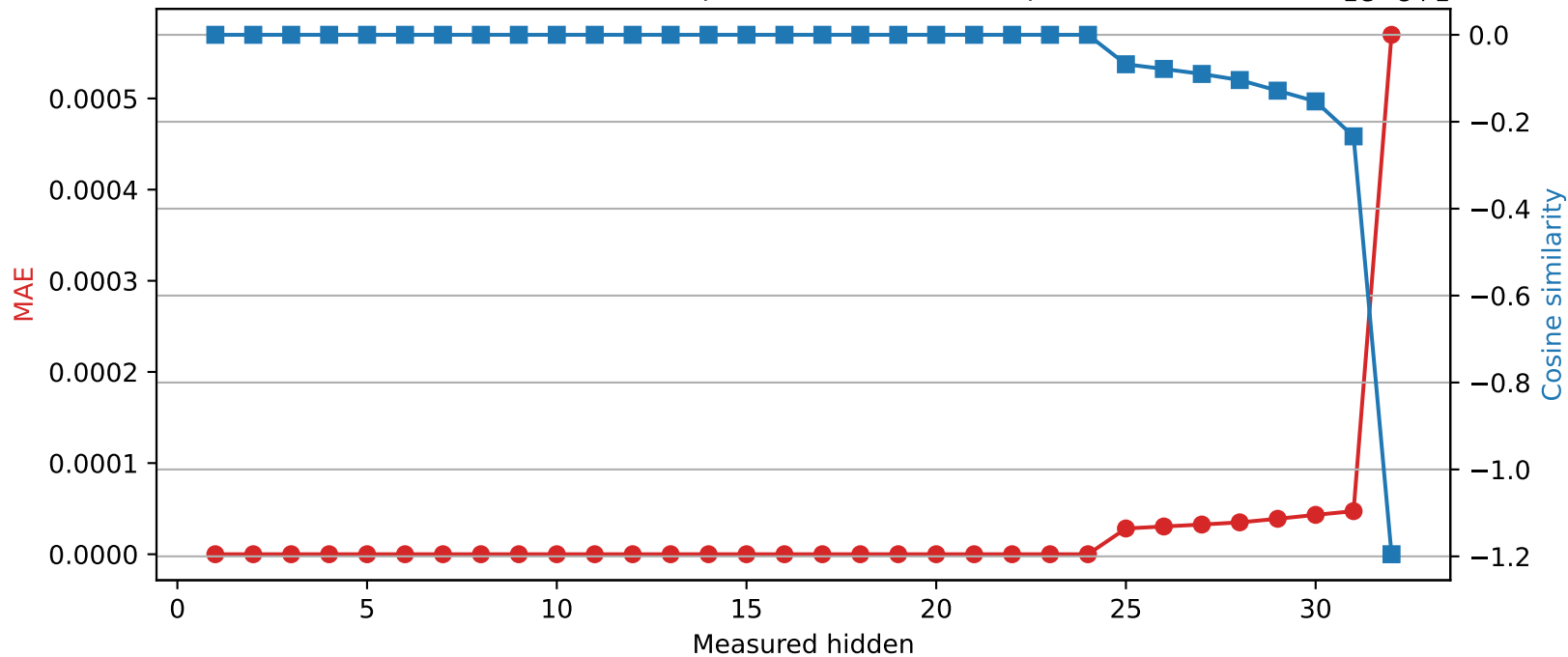
Mistral-7B-Instruct-v0.3 | Quantized layer 24 | float64 → int16
