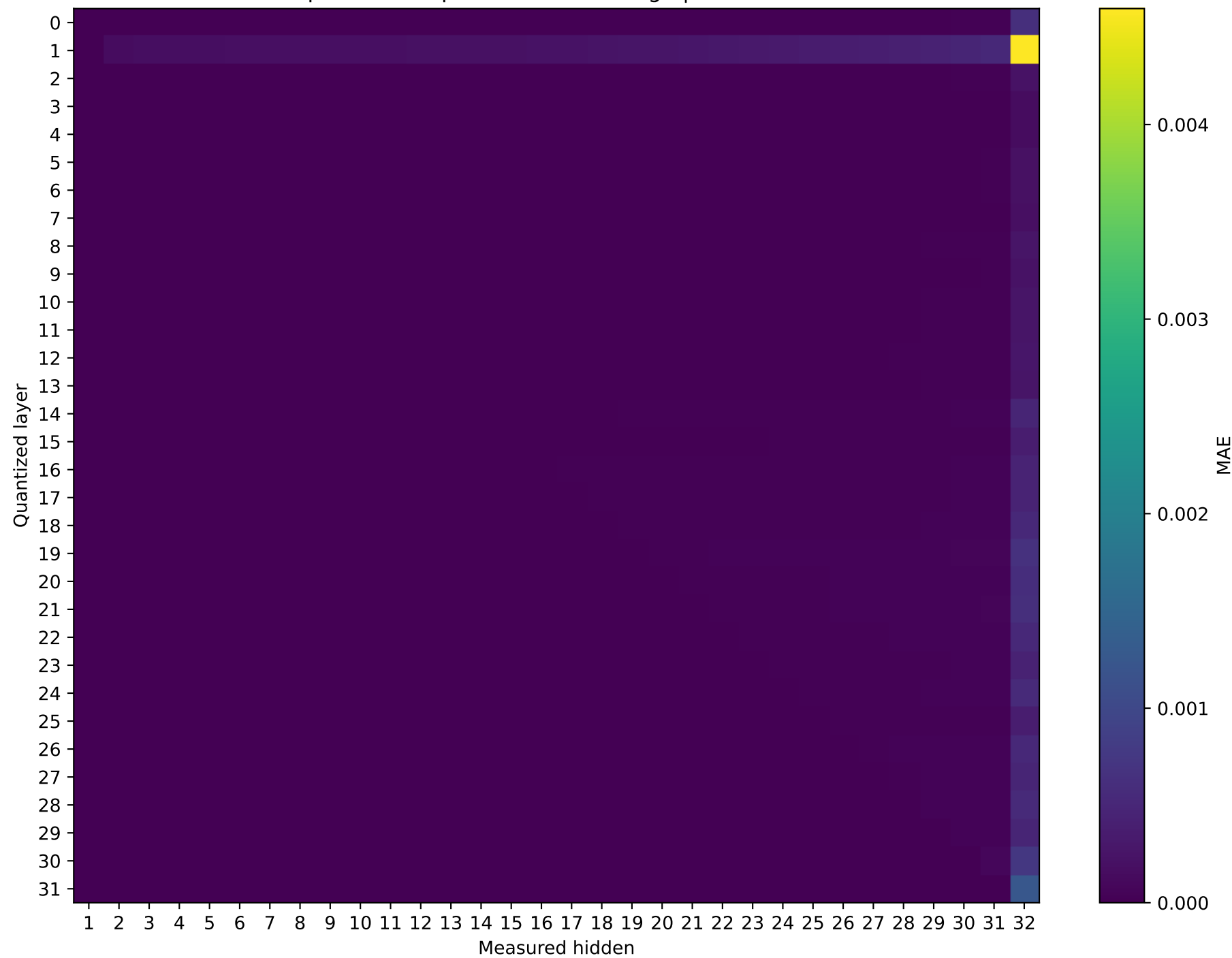
Mistral-7B-Instruct-v0.3 Prompt 2: MAE representation damage | float64 → int16
