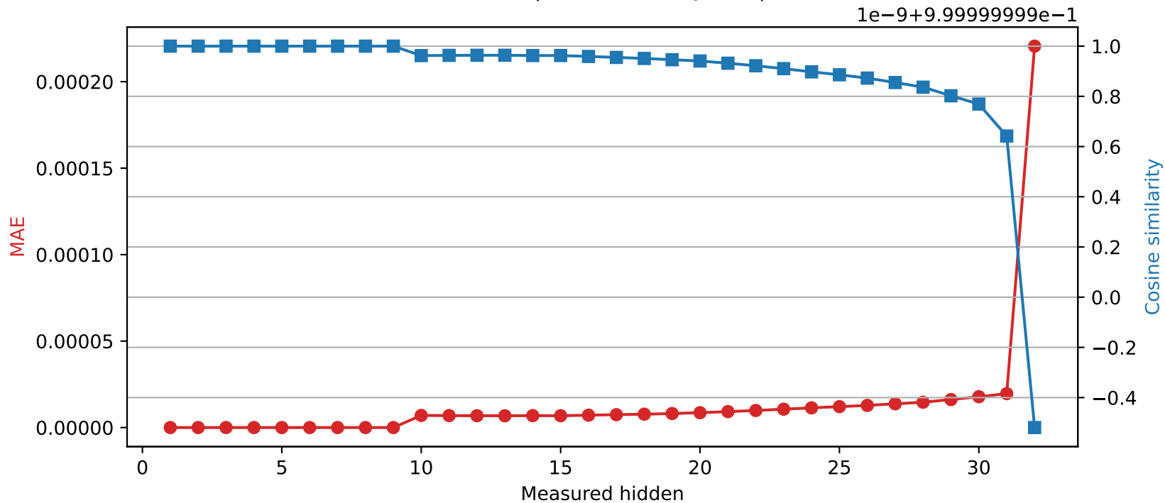
Mistral-7B-Instruct-v0.3 | Quantized layer 9 | float64 \rightarrow int16
