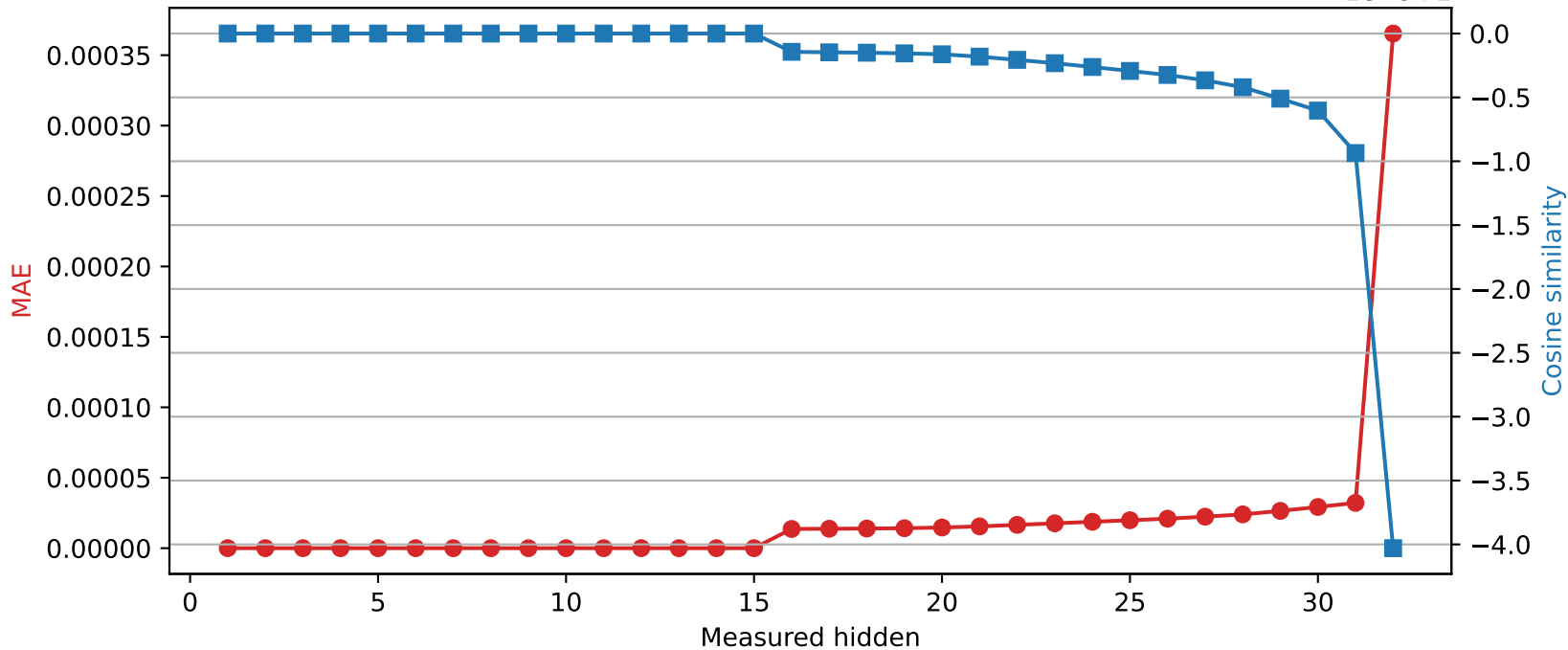
Mistral-7B-Instruct-v0.3 | Quantized layer 15 | float64 → int16
