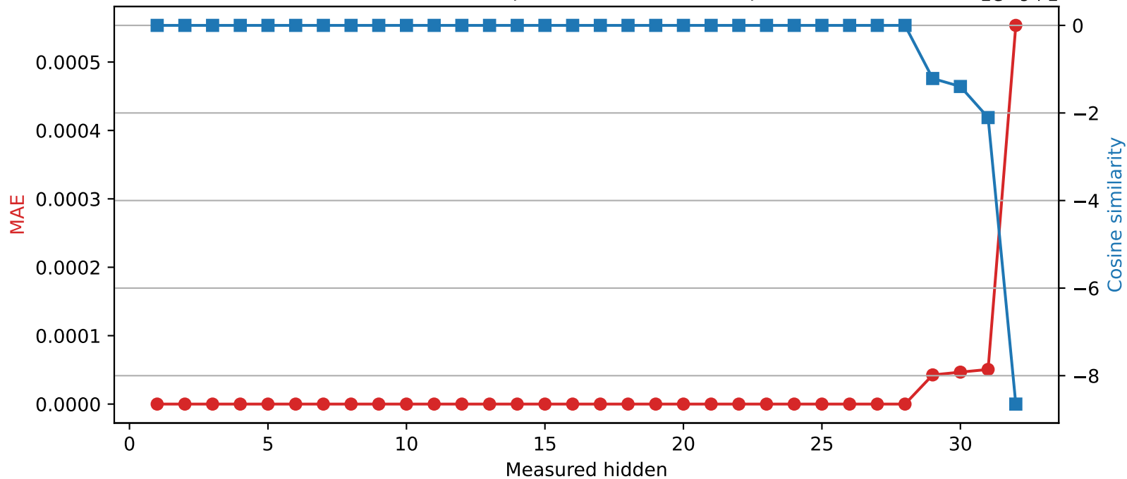
Mistral-7B-Instruct-v0.3 | Quantized layer 28 | float64 → int16
