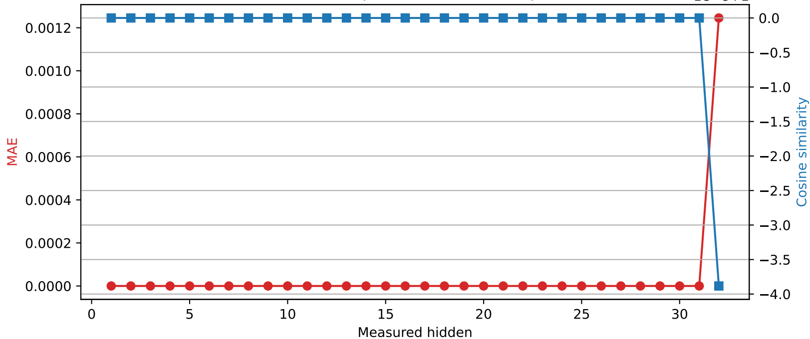
Mistral-7B-Instruct-v0.3 | Quantized layer 31 | float64 → int16
