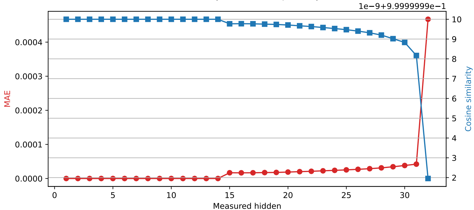
Mistral-7B-Instruct-v0.3 | Quantized layer 14 | float64 → int16
