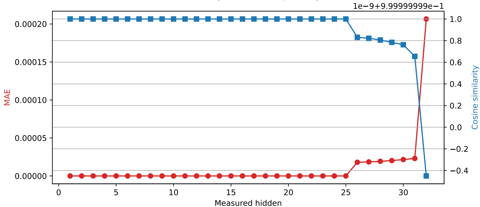
Mistral-7B-Instruct-v0.3 | Quantized layer 25 | float64 → int16
