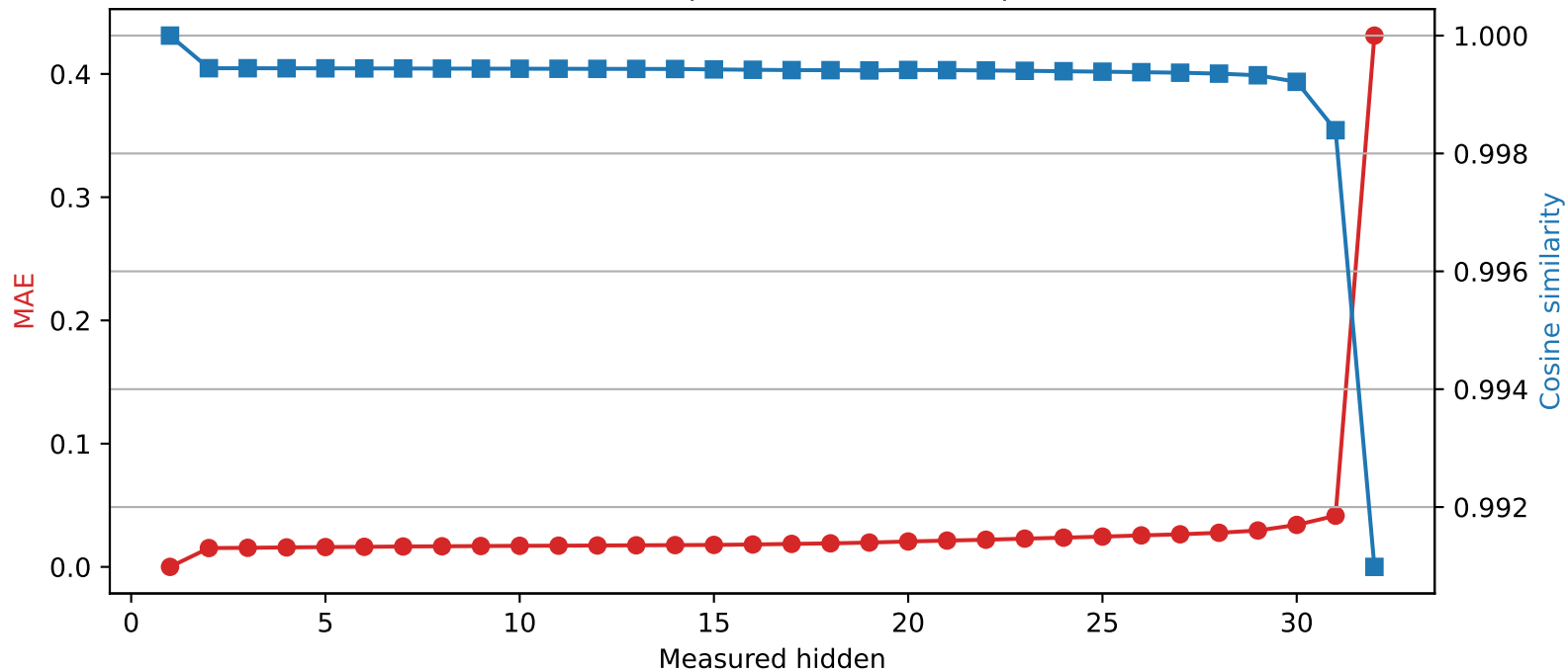
Mistral-7B-Instruct-v0.3 | Quantized layer 1 | float16 \rightarrow int8
