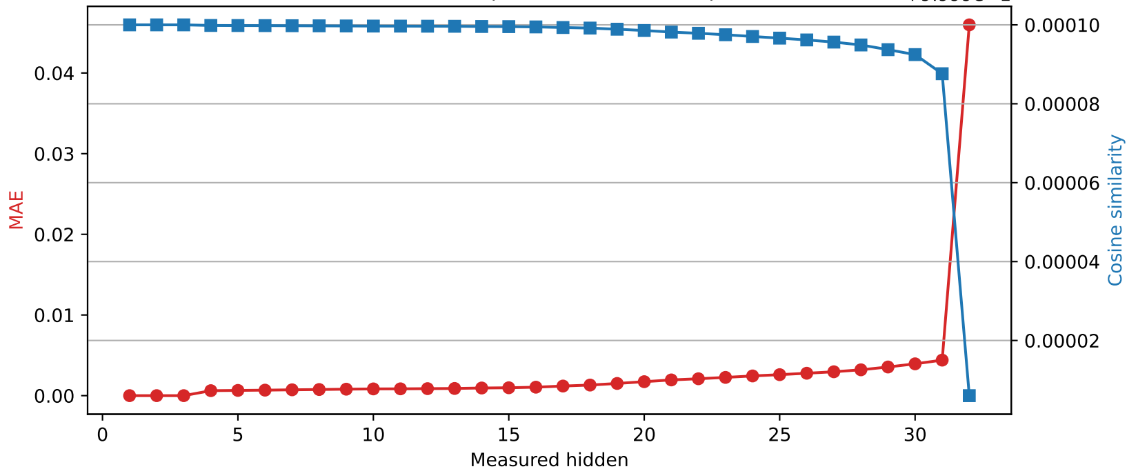
Mistral-7B-Instruct-v0.3 | Quantized layer 3 | float16 → int8
