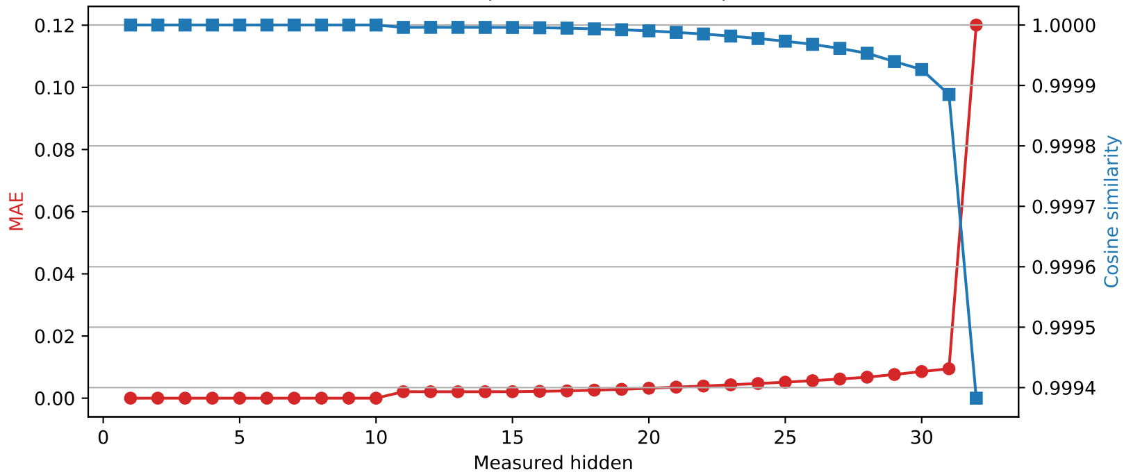
Mistral-7B-Instruct-v0.3 | Quantized layer 10 | float16 → int8
