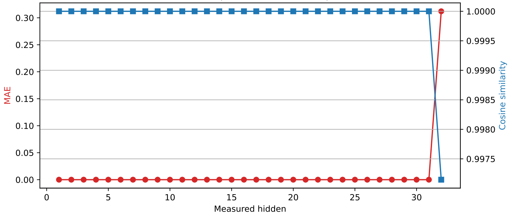
Mistral-7B-Instruct-v0.3 | Quantized layer 31 | float16 \rightarrow int8
