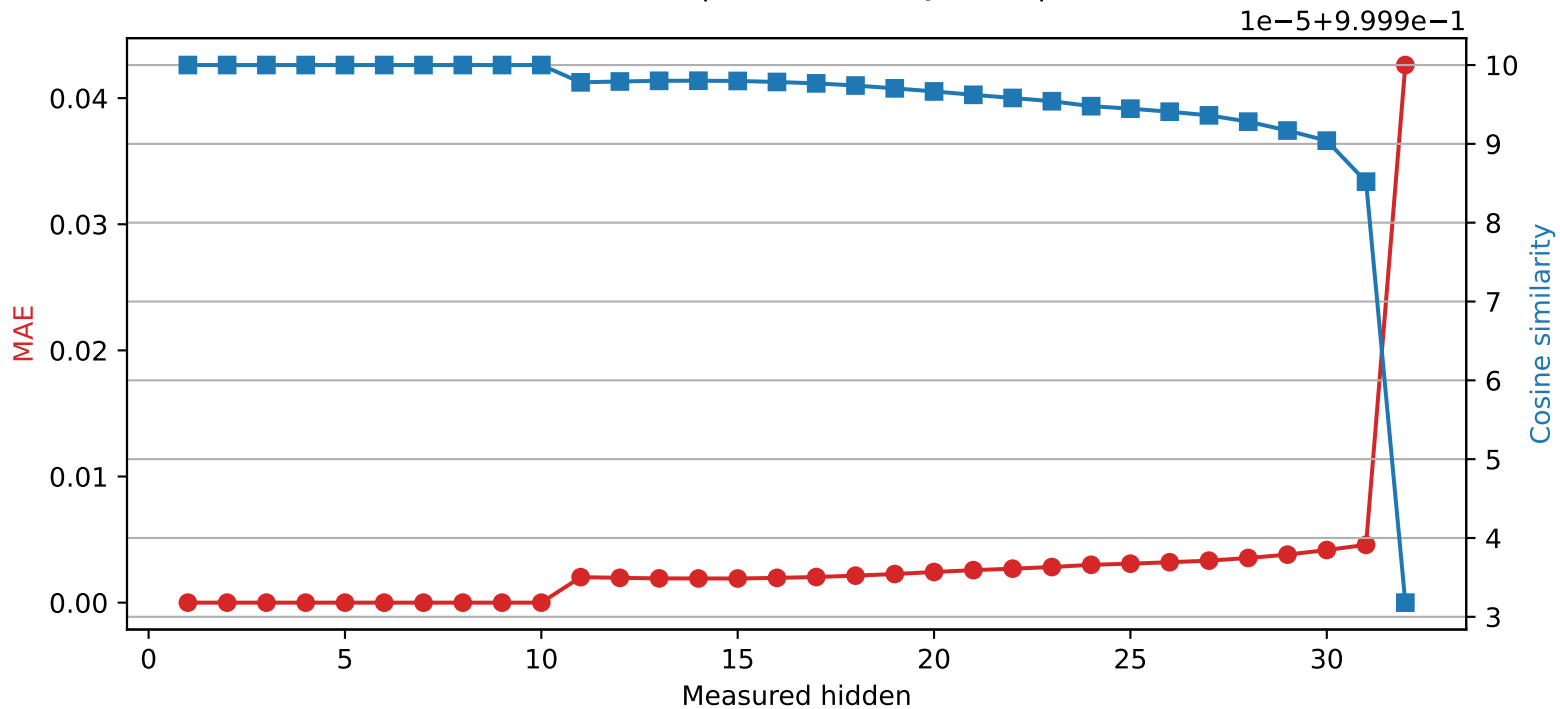
Mistral-7B-Instruct-v0.3 | Quantized layer 10 | float16 \rightarrow int8
