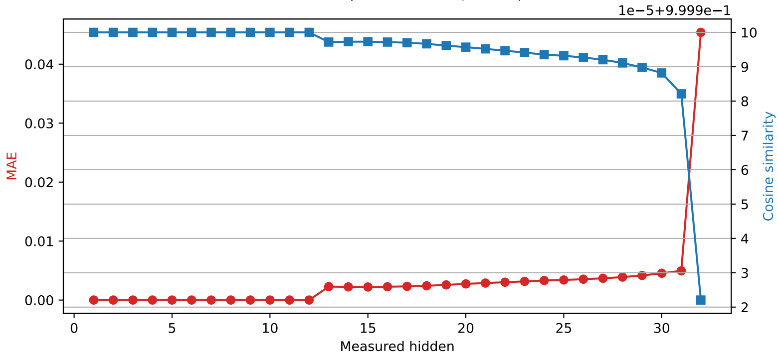
Mistral-7B-Instruct-v0.3 | Quantized layer 12 | float16 \rightarrow int8
