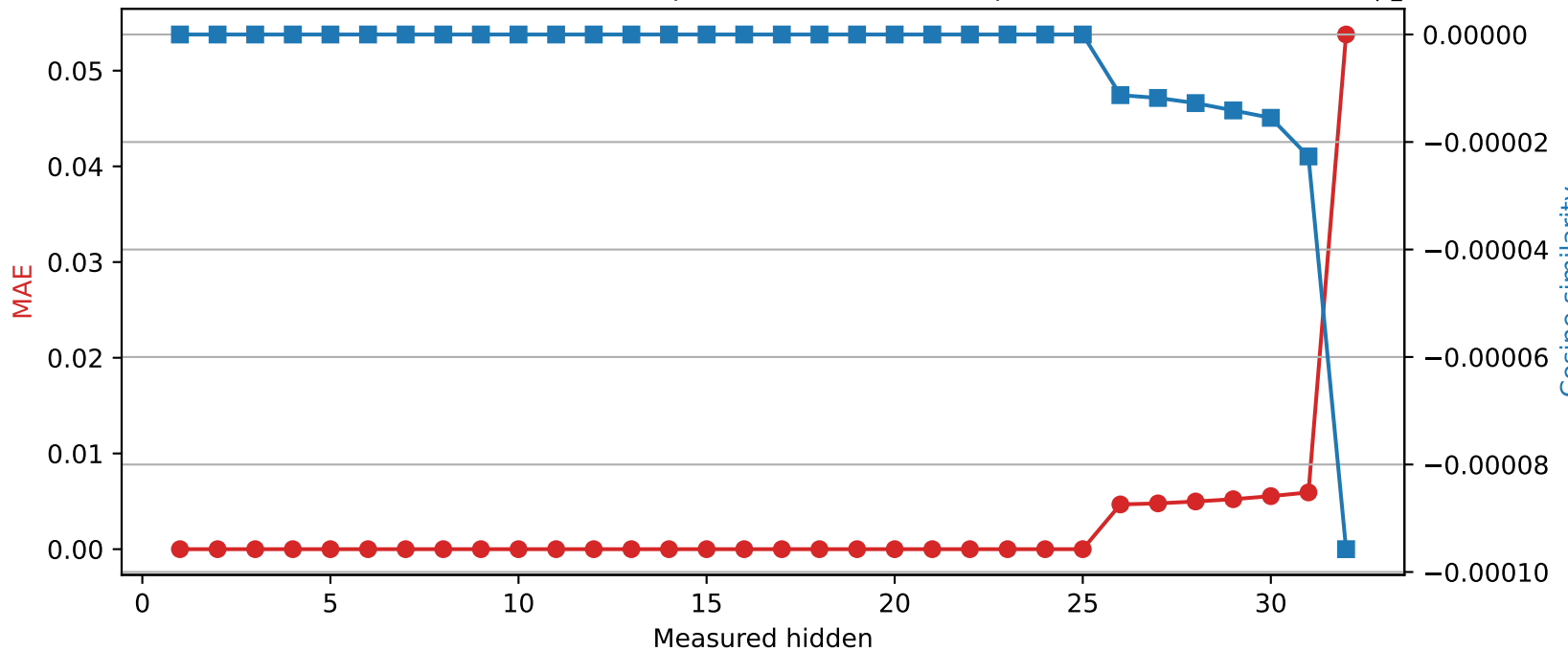
Mistral-7B-Instruct-v0.3 | Quantized layer 25 | float16 → int8
