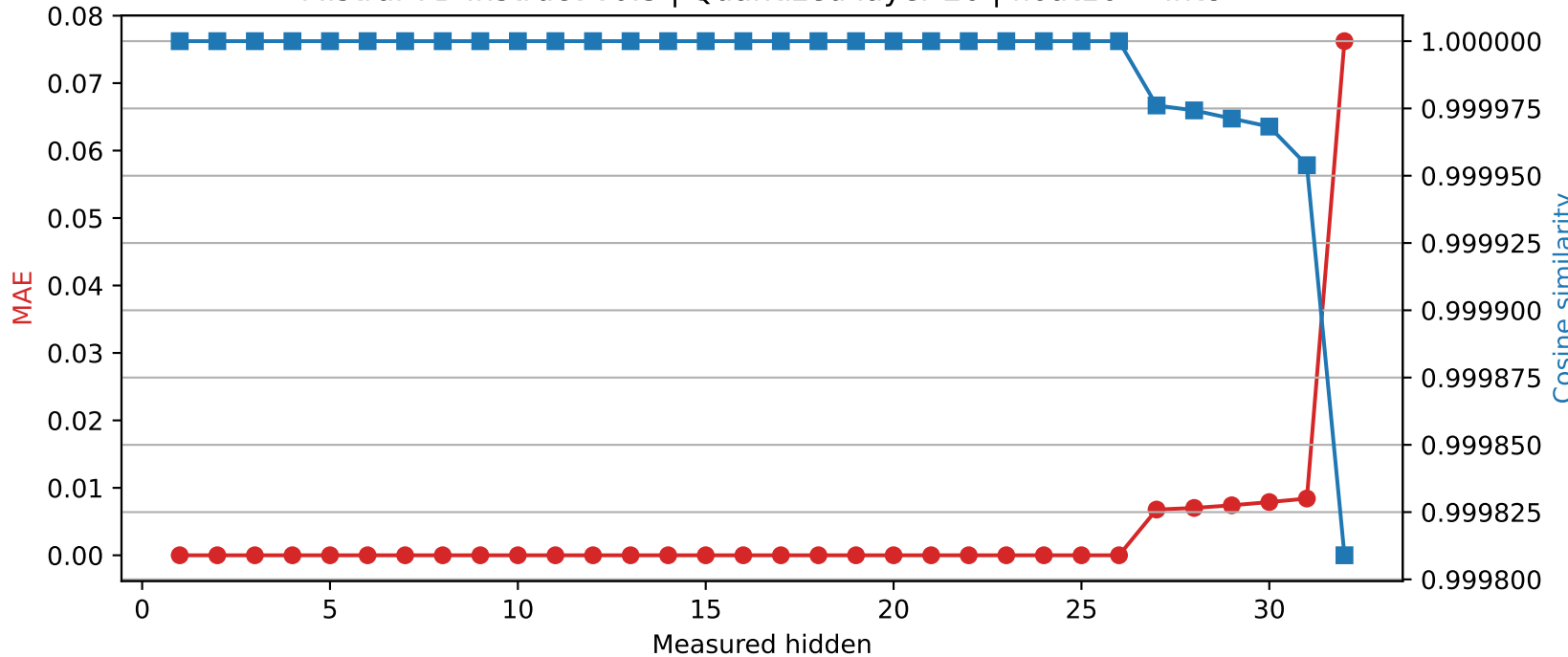
Mistral-7B-Instruct-v0.3 | Quantized layer 26 | float16 → int8
