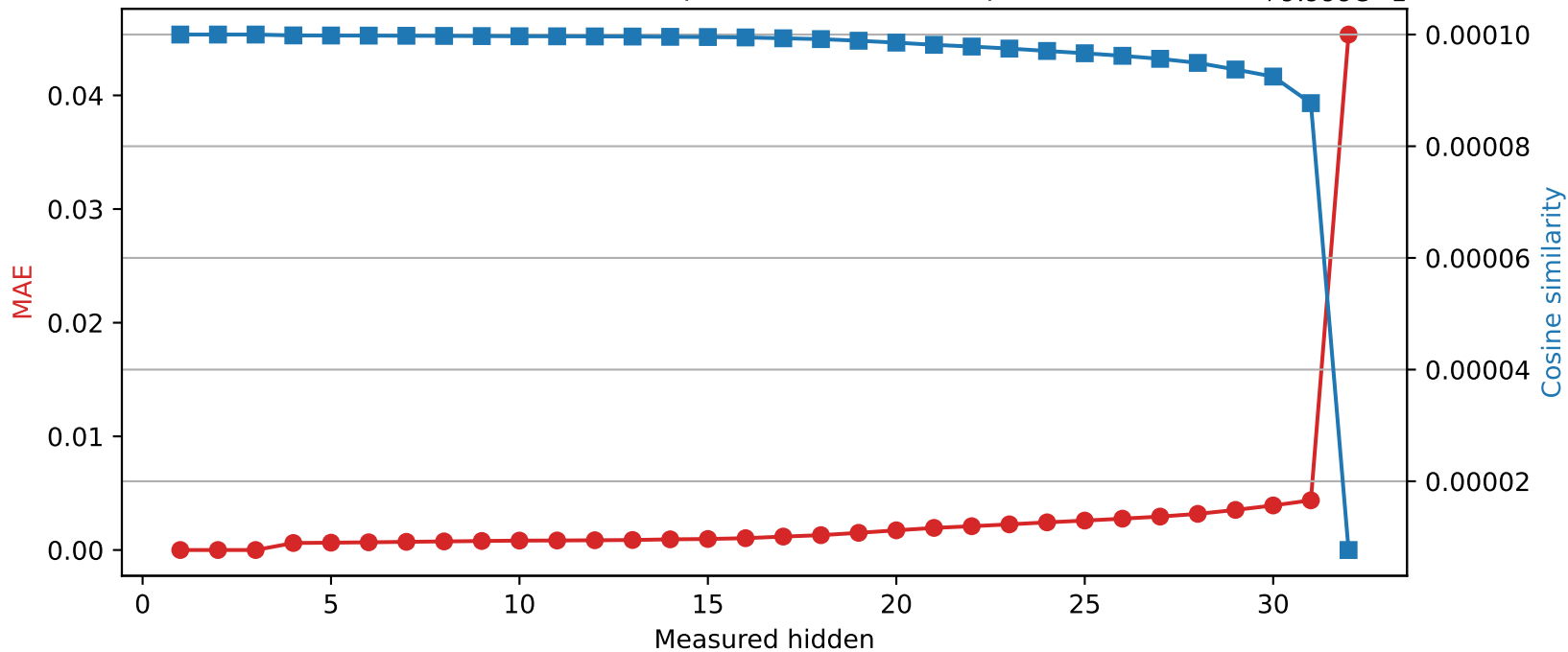
Mistral-7B-Instruct-v0.3 | Quantized layer 3 | float32 → int8
