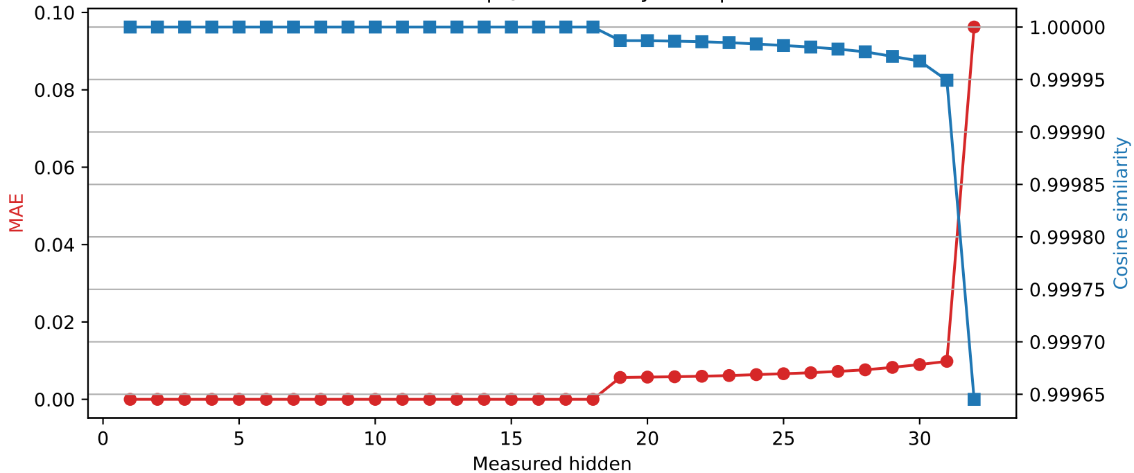
Mistral-7B-Instruct-v0.3 | Quantized layer 18 | float32 → int8
