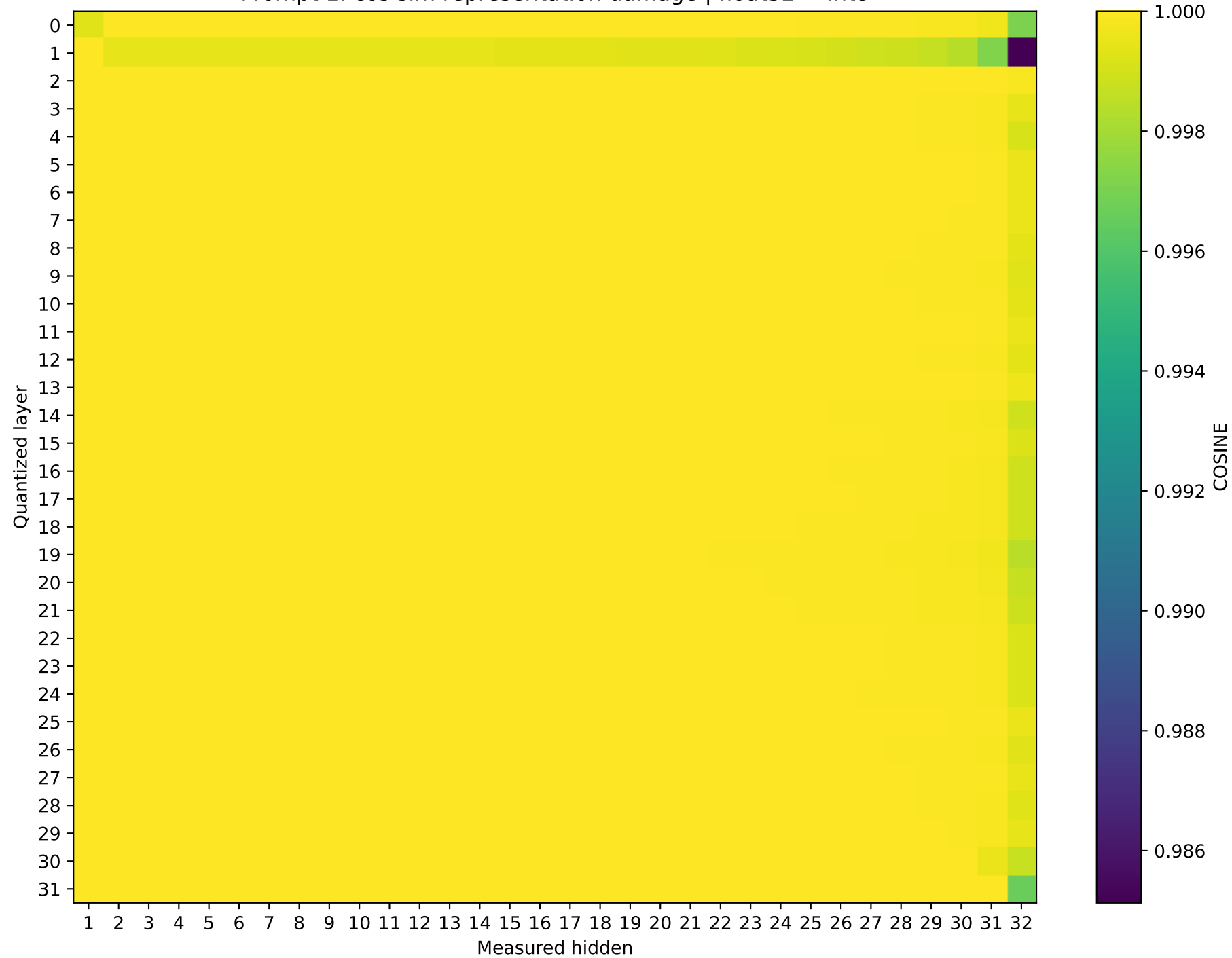
Mistral-7B-Instruct-v0.3 Prompt 1: cos sim representation damage | float32 → int8
