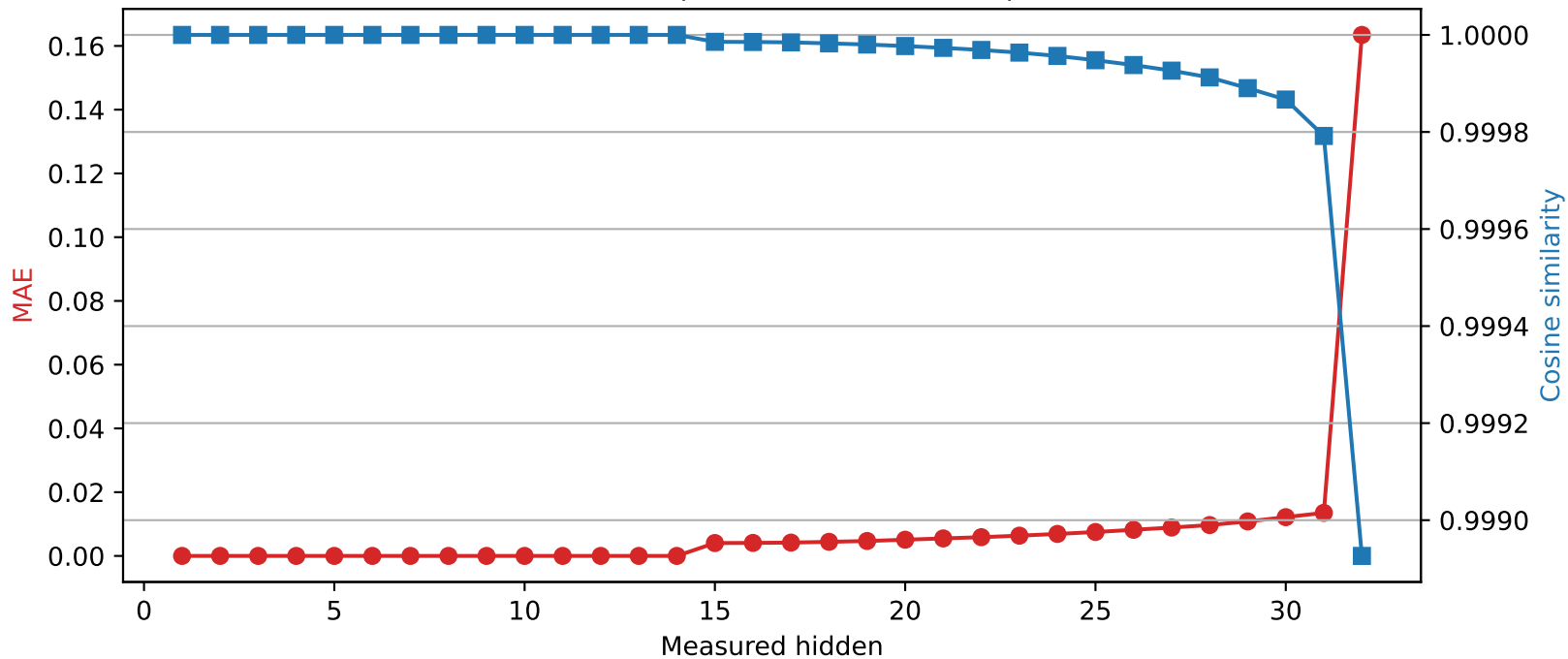
Mistral-7B-Instruct-v0.3 | Quantized layer 14 | float32 → int8
