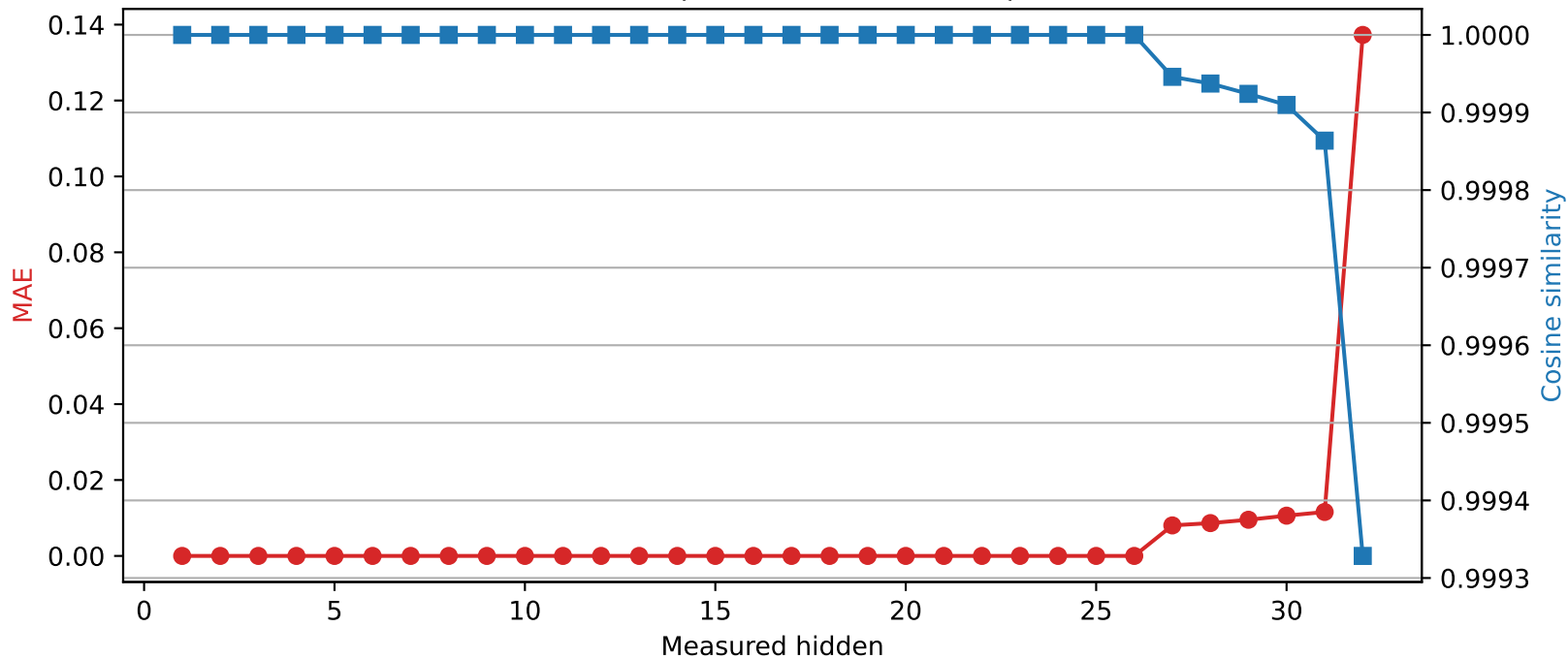
Mistral-7B-Instruct-v0.3 | Quantized layer 26 | float32 → int8
