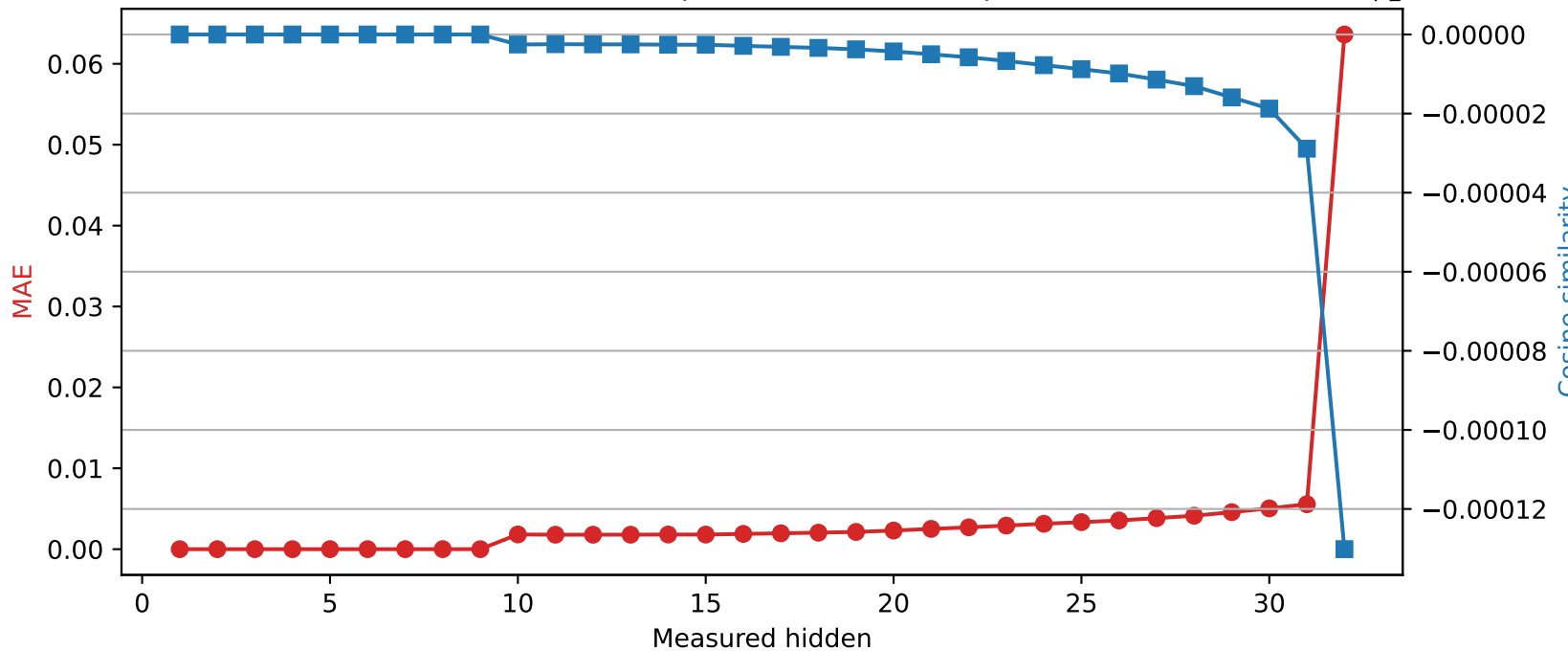
Mistral-7B-Instruct-v0.3 | Quantized layer 9 | float32 → int8
