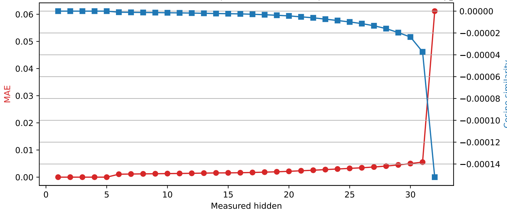
Mistral-7B-Instruct-v0.3 | Quantized layer 5 | float32 → int8
