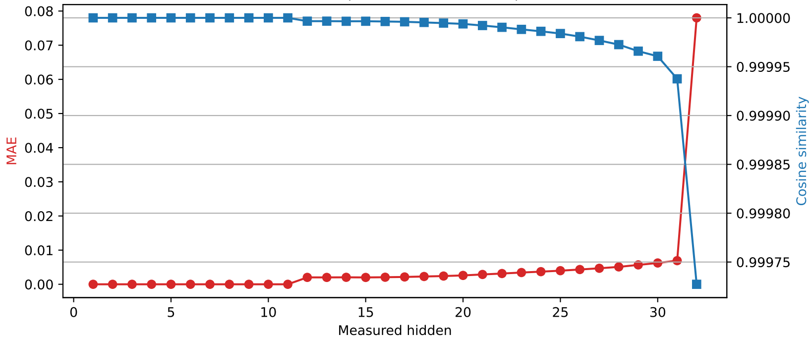
Mistral-7B-Instruct-v0.3 | Quantized layer 11 | float32 \rightarrow int8
