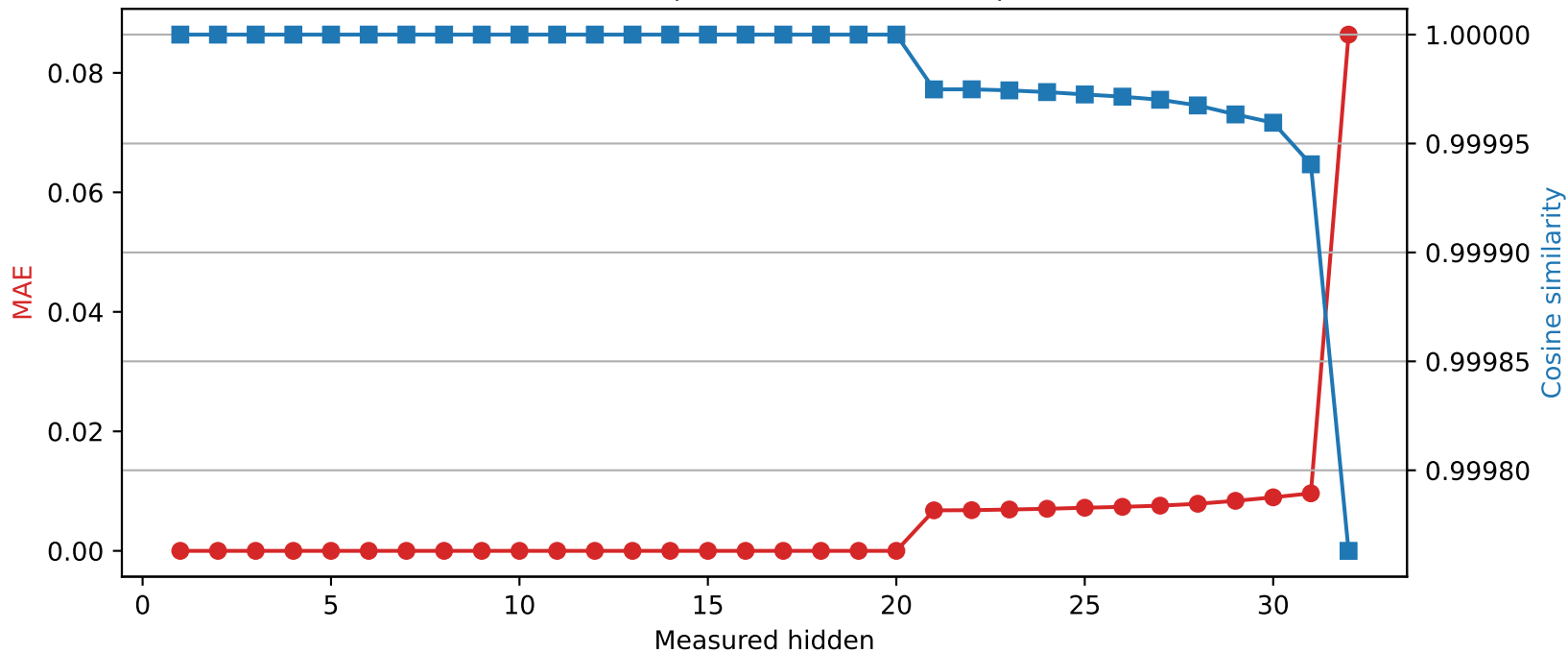
Mistral-7B-Instruct-v0.3 | Quantized layer 20 | float32 → int8
