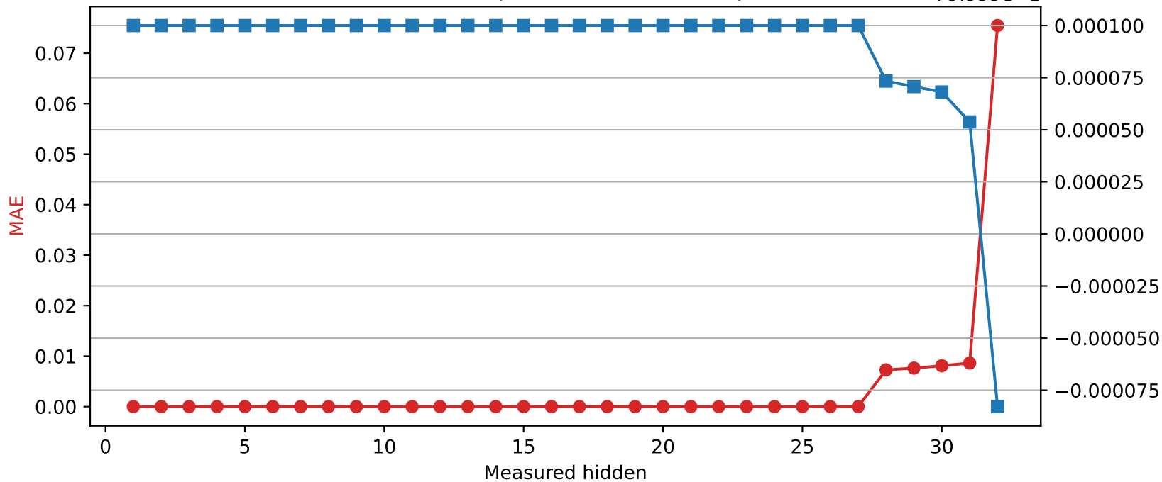
Mistral-7B-Instruct-v0.3 | Quantized layer 27 | float32 → int8 +9.999e-1
