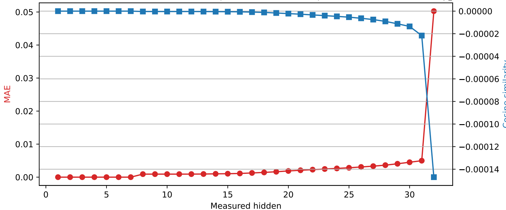
Mistral-7B-Instruct-v0.3 | Quantized layer 7 | float64 → int8
