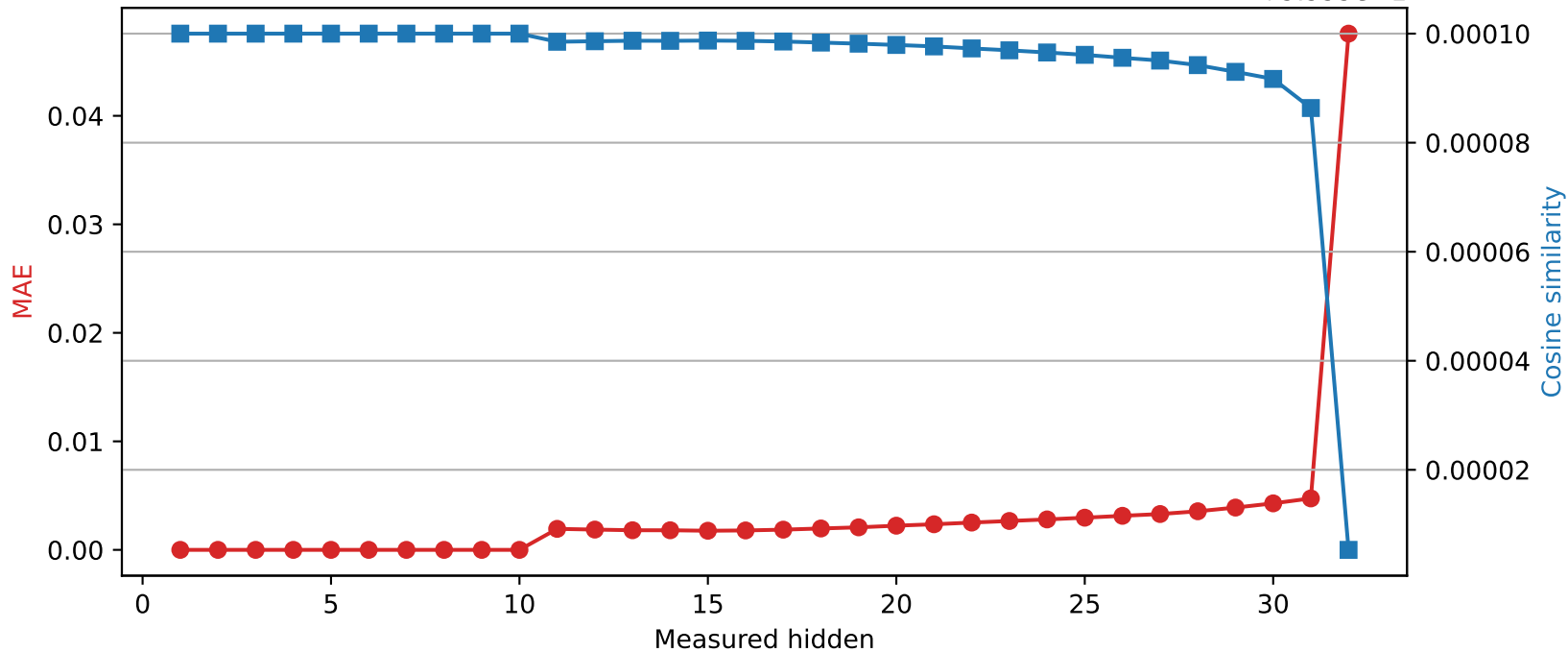
Mistral-7B-Instruct-v0.3 | Quantized layer 10 | float64 → int8 +9.999e-1
