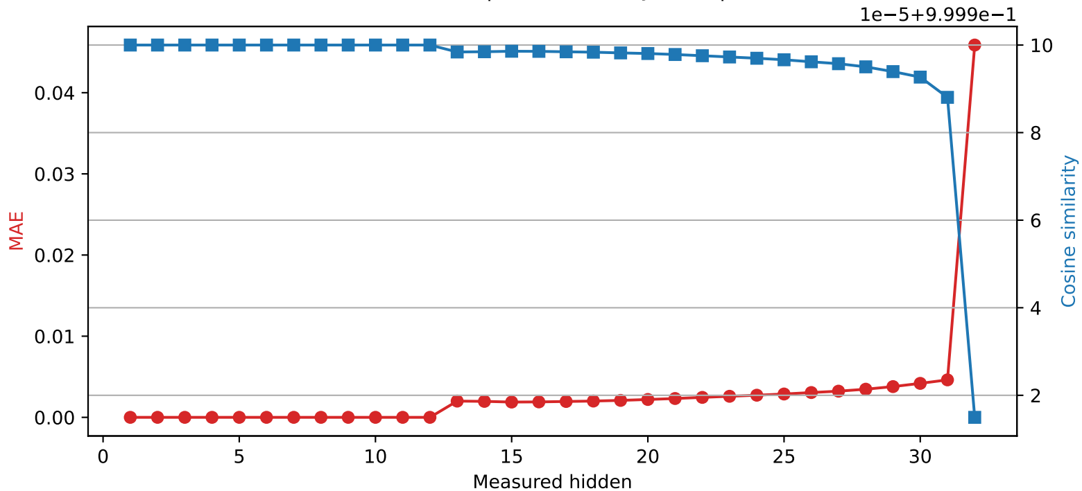
Mistral-7B-Instruct-v0.3 | Quantized layer 12 | float64 → int8
