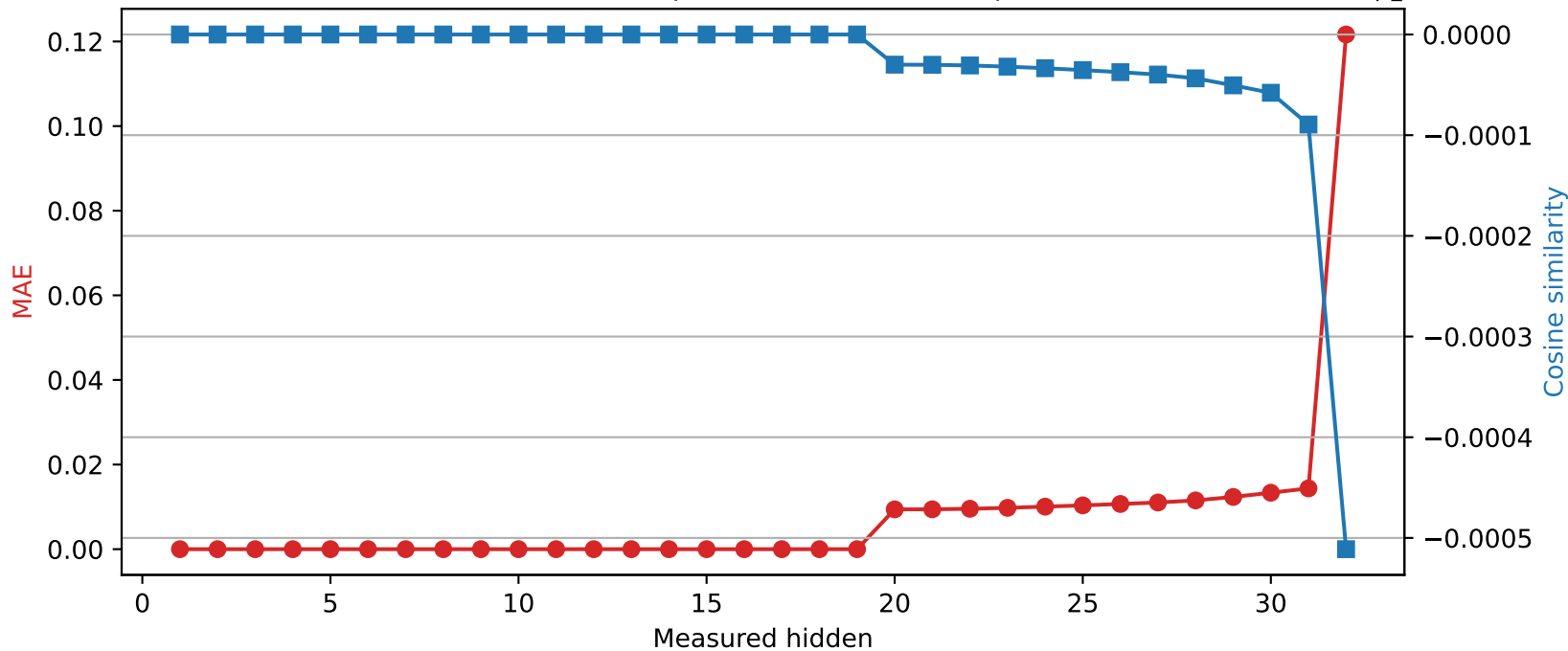
Mistral-7B-Instruct-v0.3 | Quantized layer 19 | float64 → int8
