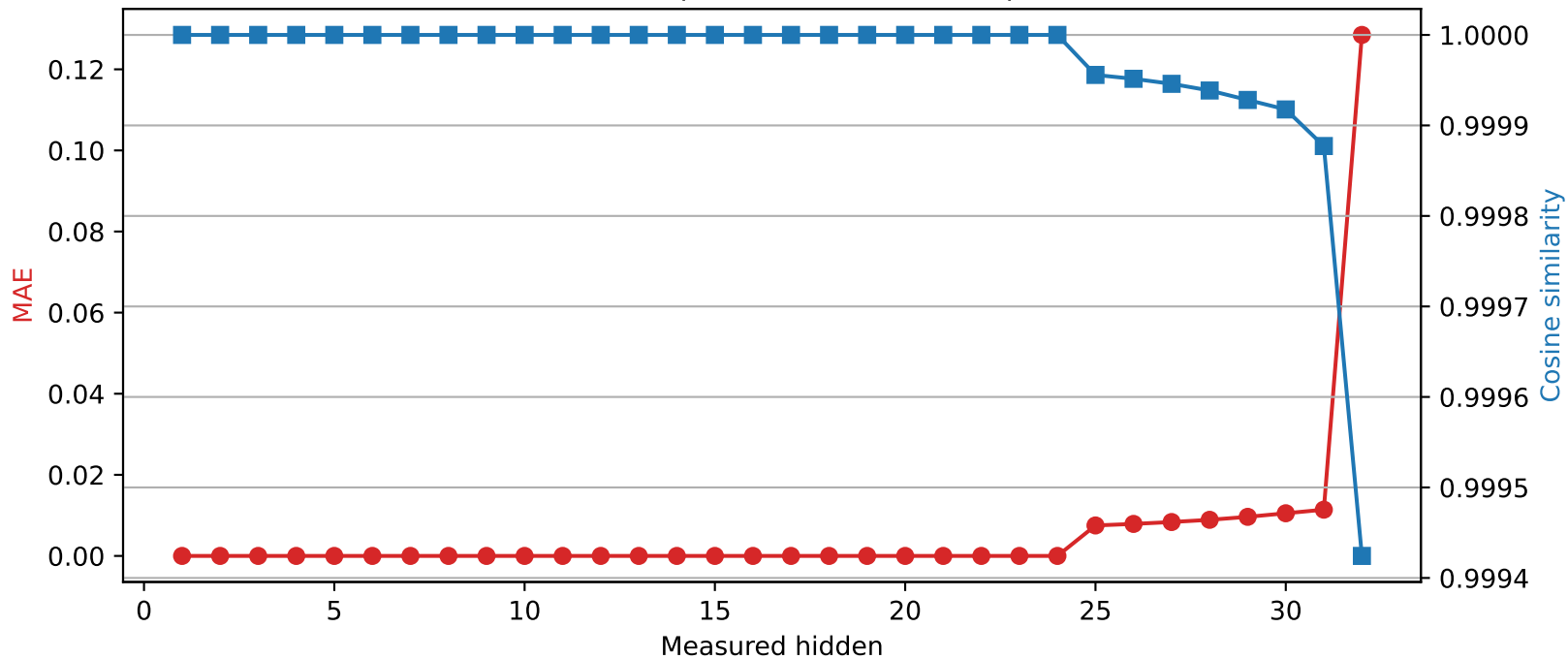
Mistral-7B-Instruct-v0.3 | Quantized layer 24 | float64 → int8
