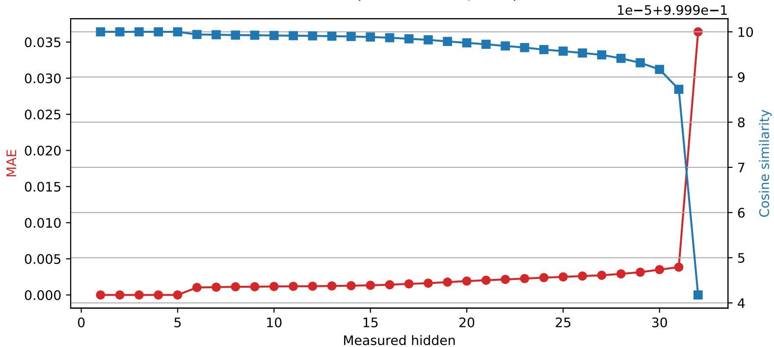
Mistral-7B-Instruct-v0.3 | Quantized layer 5 | float64 → int8
