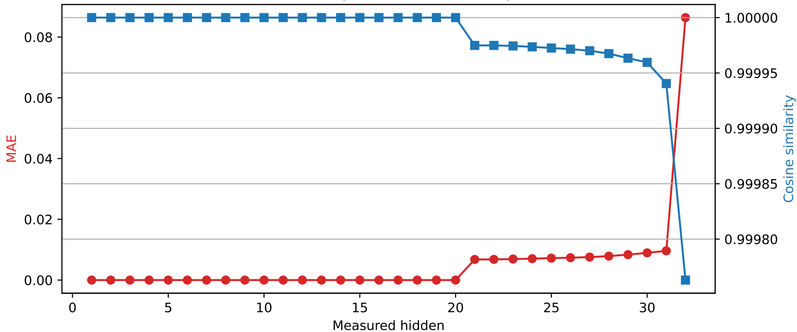
Mistral-7B-Instruct-v0.3 | Quantized layer 20 | float64 → int8
