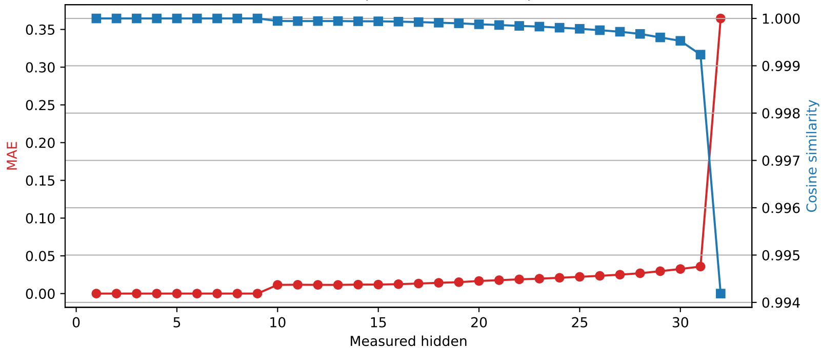
Mistral-7B-Instruct-v0.3 | Quantized layer 9 | float16 → int4
