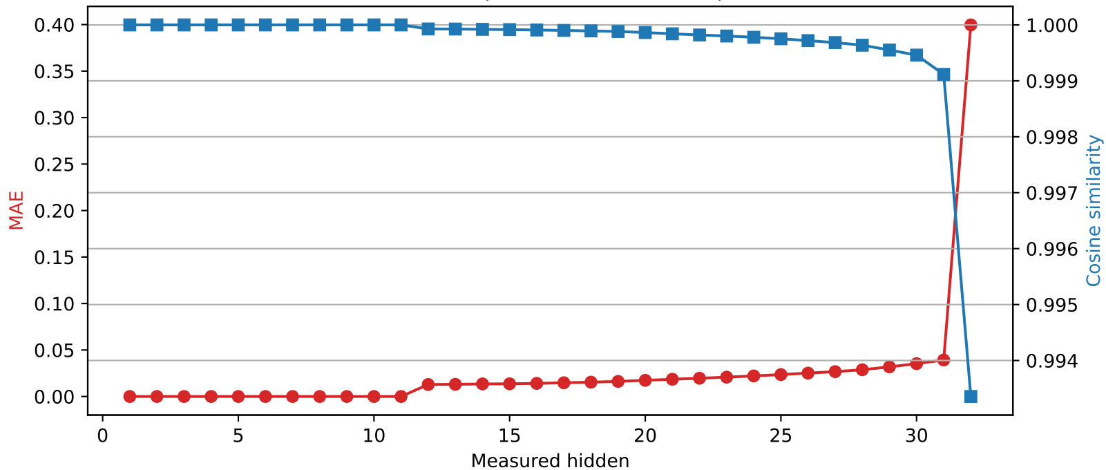
Mistral-7B-Instruct-v0.3 | Quantized layer 11 | float16 \rightarrow int4
