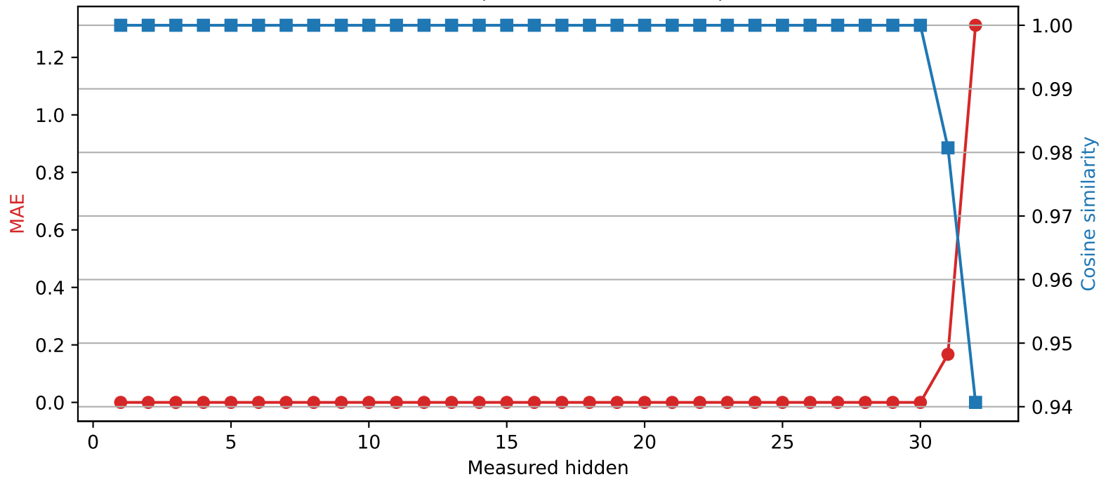
Mistral-7B-Instruct-v0.3 | Quantized layer 30 | float16 → int4
