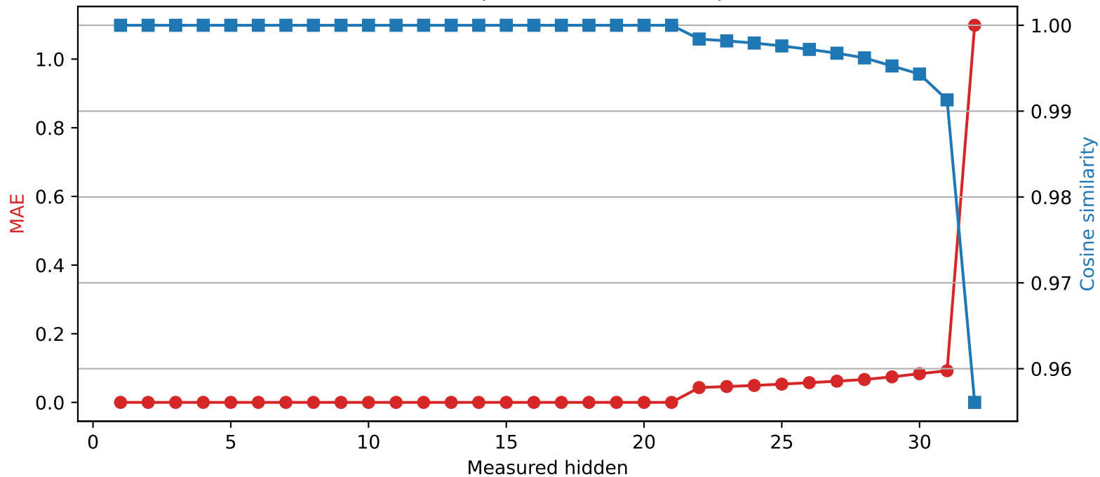
Mistral-7B-Instruct-v0.3 | Quantized layer 21 | float16 → int4
